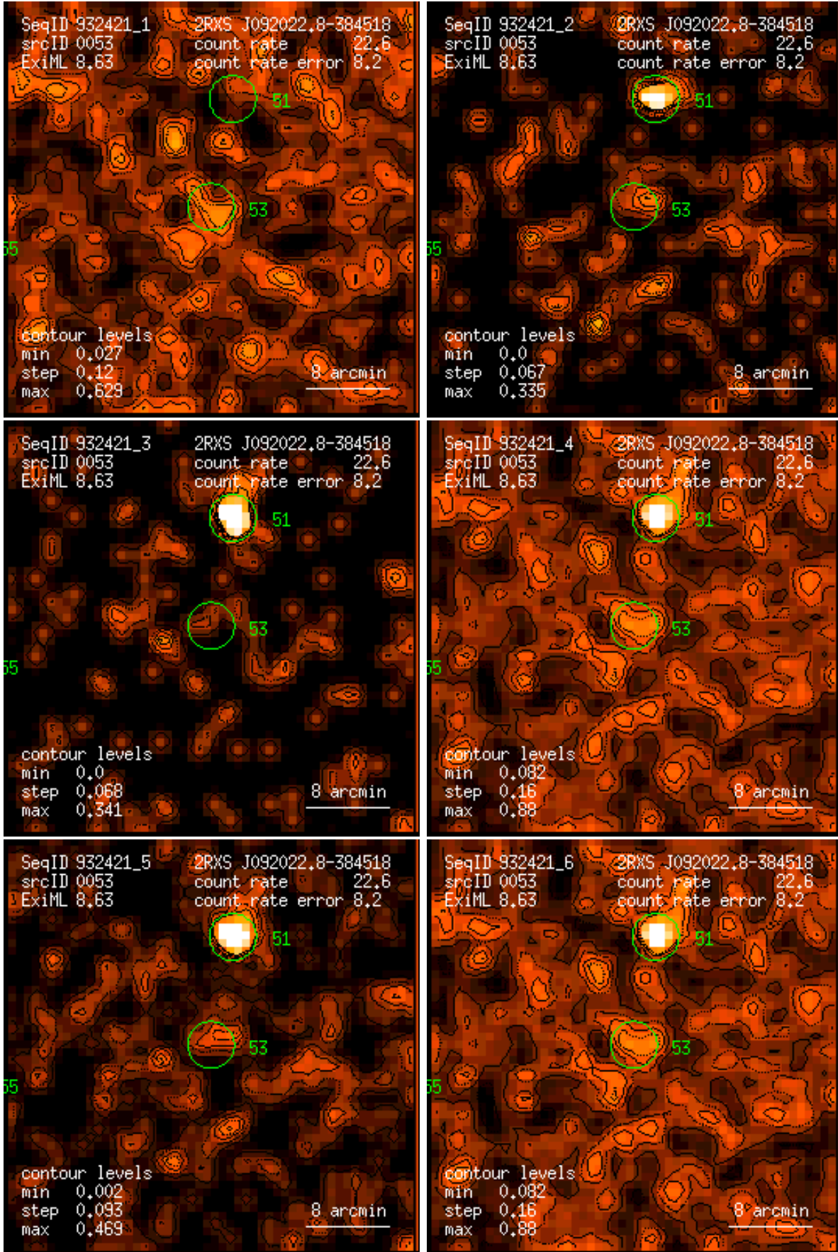
Figure 53: RASS 932421: detection 0053: band rate images, Gaussian filter: (1) PSPC channels 11 – 41, (2) 52 – 90, (3) 91 – 201, (4) 11 – 235, (5) 52 – 201, (6) 11 – 201. Broad band rates in counts/ks. Band rate contour levels in counts/ks/arcmin 2 .
