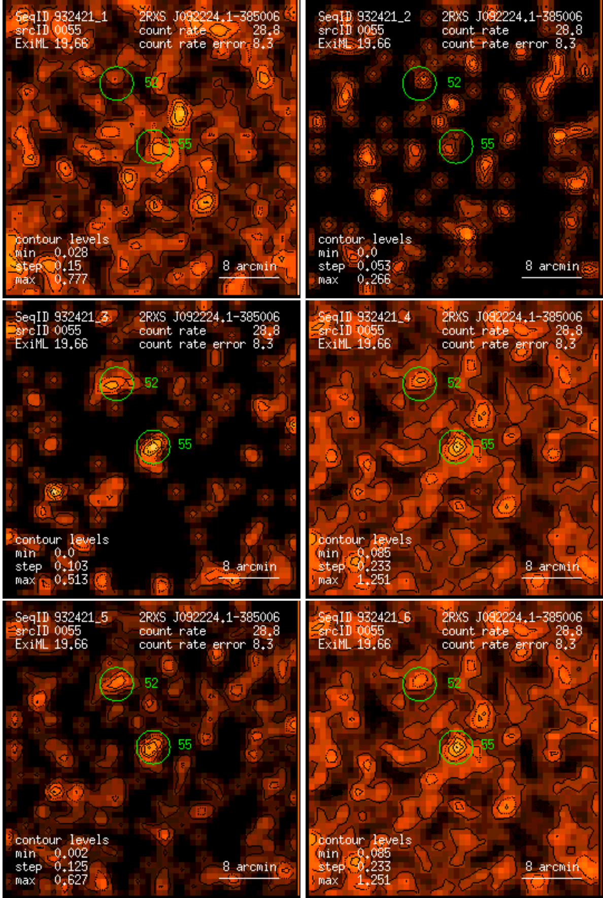
Figure 55: RASS 932421: detection 0055: band rate images, Gaussian filter: (1) PSPC channels 11 – 41, (2) 52 – 90, (3) 91 – 201, (4) 11 – 235, (5) 52 – 201, (6) 11 – 201. Broad band rates in counts/ks. Band rate contour levels in counts/ks/arcmin 2 .
