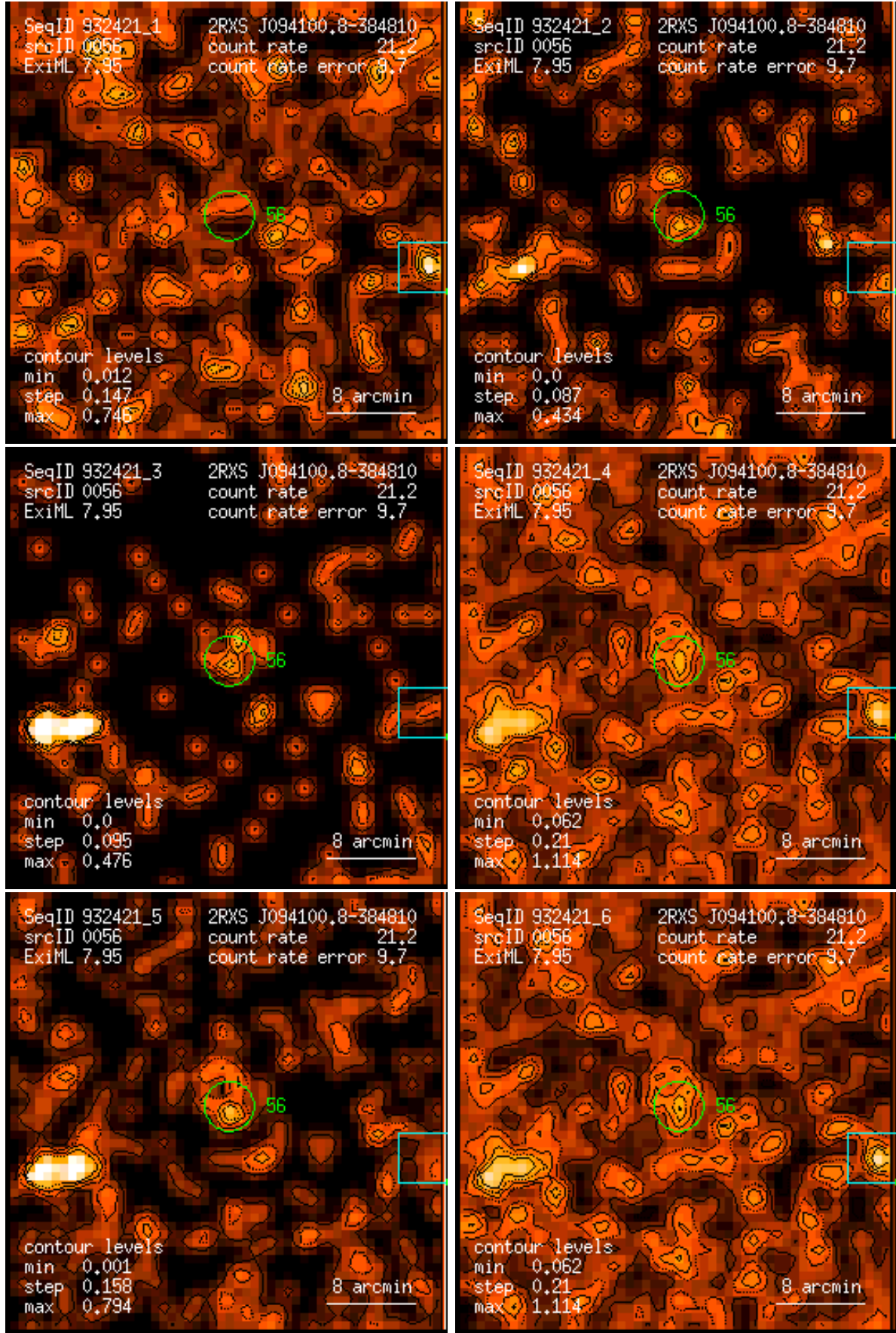
Figure 56: RASS 932421: detection 0056: band rate images, Gaussian filter: (1) PSPC channels 11 – 41, (2) 52 – 90, (3) 91 – 201, (4) 11 – 235, (5) 52 – 201, (6) 11 – 201. Broad band rates in counts/ks. Band rate contour levels in counts/ks/arcmin 2 .
