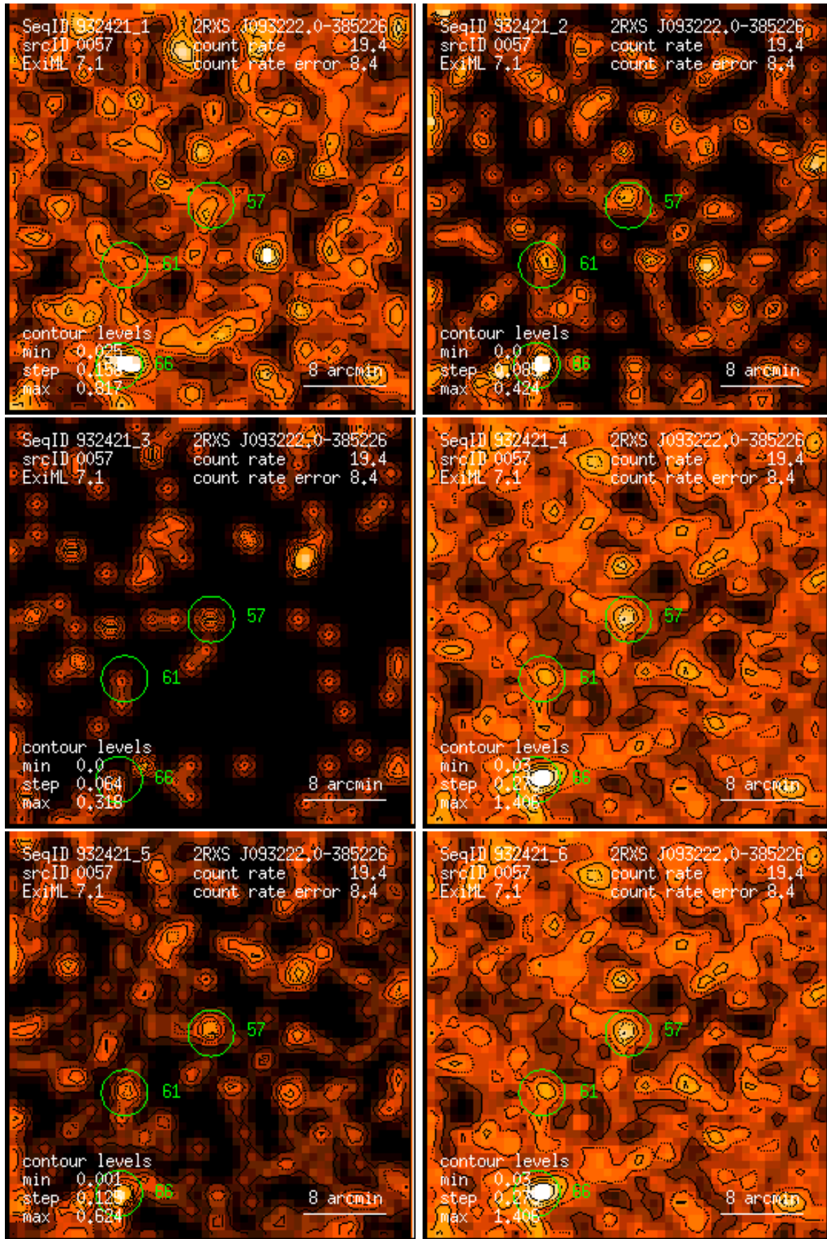
Figure 57: RASS 932421: detection 0057: band rate images, Gaussian filter: (1) PSPC channels 11 – 41, (2) 52 – 90, (3) 91 – 201, (4) 11 – 235, (5) 52 – 201, (6) 11 – 201. Broad band rates in counts/ks. Band rate contour levels in counts/ks/arcmin 2 .
