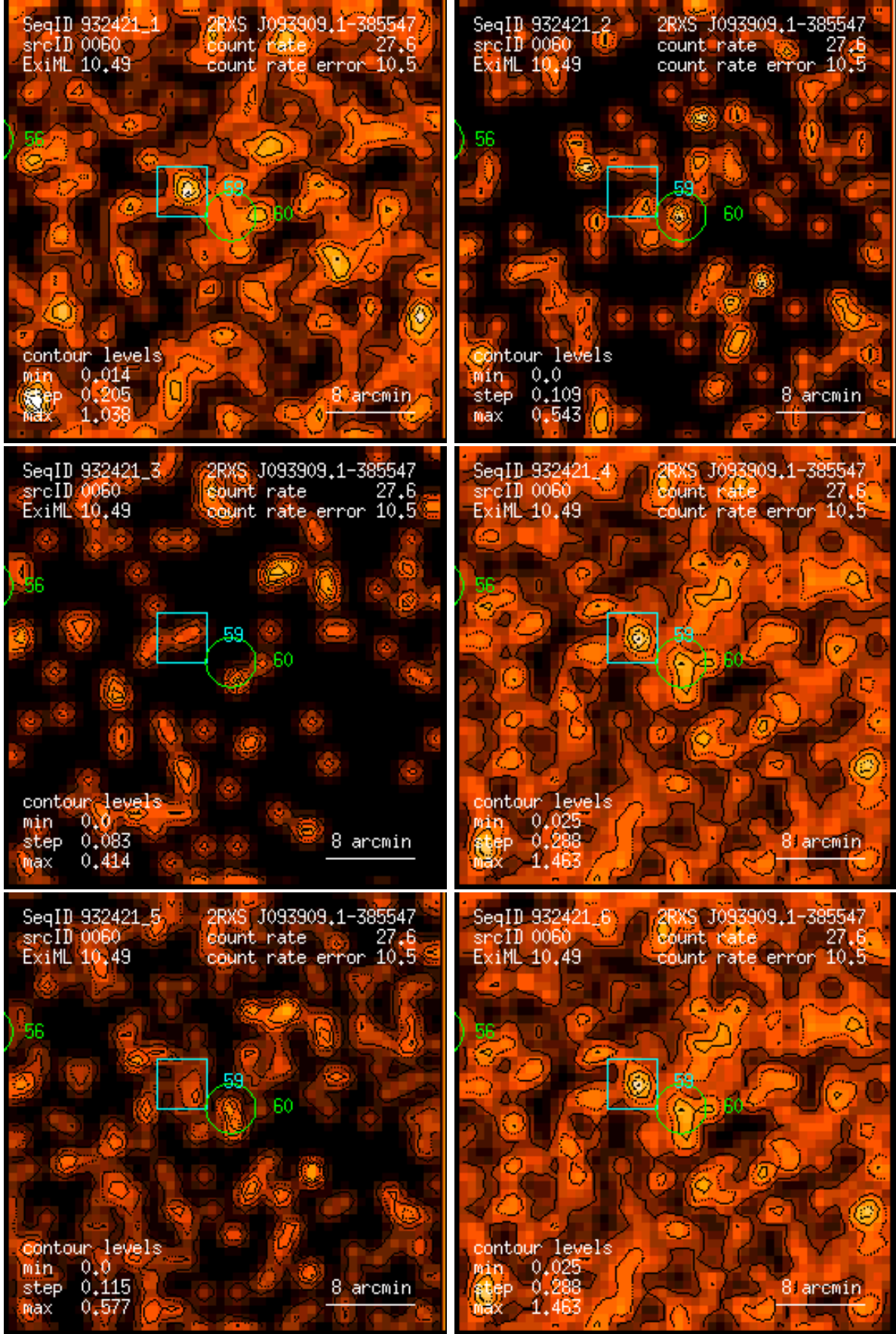
Figure 60: RASS 932421: detection 0060: band rate images, Gaussian filter: (1) PSPC channels 11 – 41, (2) 52 – 90, (3) 91 – 201, (4) 11 – 235, (5) 52 – 201, (6) 11 – 201. Broad band rates in counts/ks. Band rate contour levels in counts/ks/arcmin 2 .
