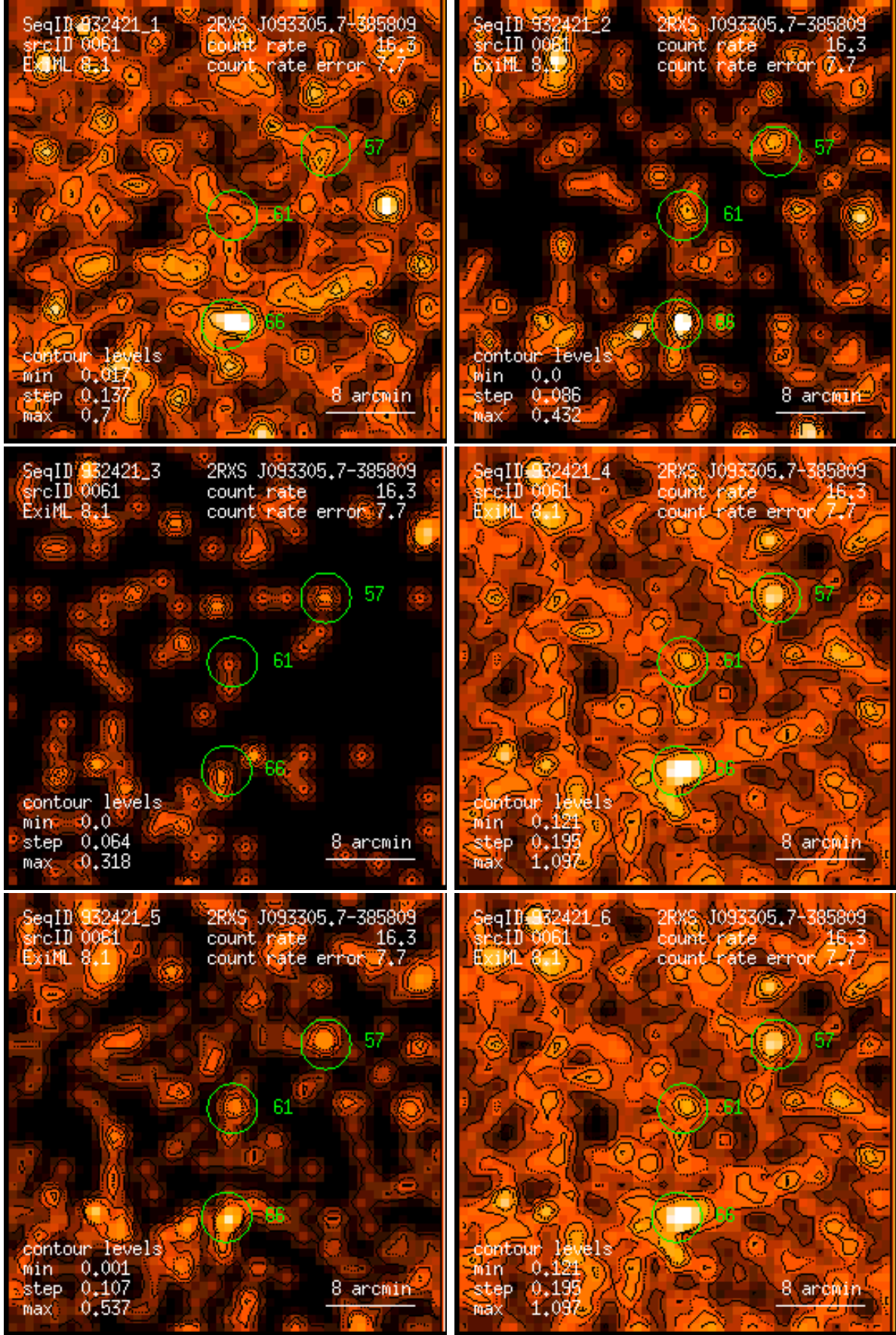
Figure 61: RASS 932421: detection 0061: band rate images, Gaussian filter: (1) PSPC channels 11 – 41, (2) 52 – 90, (3) 91 – 201, (4) 11 – 235, (5) 52 – 201, (6) 11 – 201. Broad band rates in counts/ks. Band rate contour levels in counts/ks/arcmin 2 .
