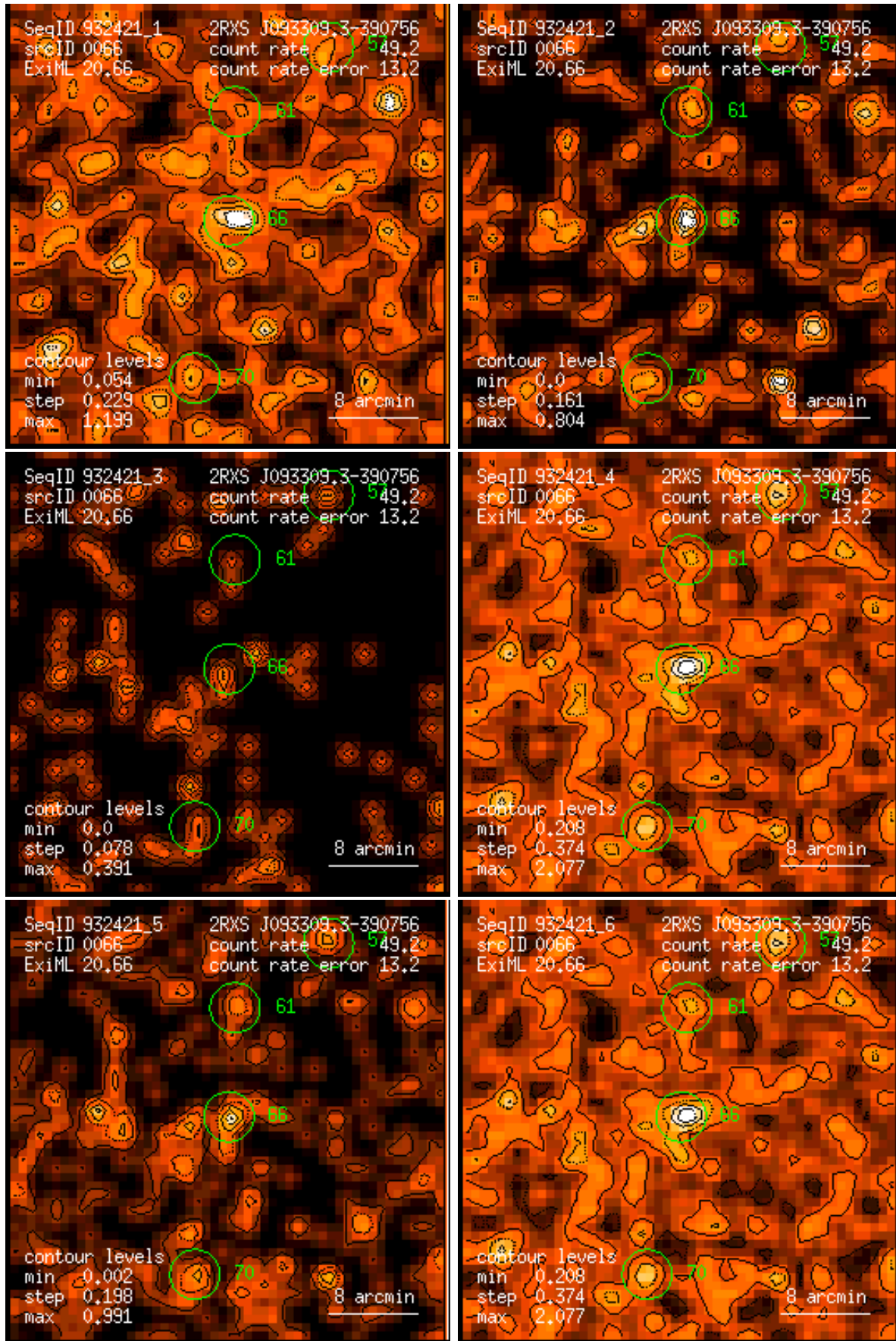
Figure 66: RASS 932421: detection 0066: band rate images, Gaussian filter: (1) PSPC channels 11 – 41, (2) 52 – 90, (3) 91 – 201, (4) 11 – 235, (5) 52 – 201, (6) 11 – 201. Broad band rates in counts/ks. Band rate contour levels in counts/ks/arcmin 2 .
