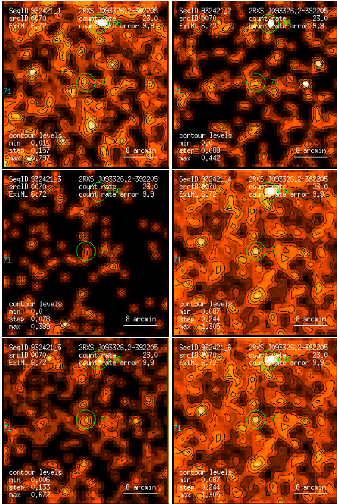
Figure 70: RASS 932421: detection 0070: band rate images, Gaussian filter: (1) PSPC channels 11 – 41, (2) 52 – 90, (3) 91 – 201, (4) 11 – 235, (5) 52 – 201, (6) 11 – 201. Broad band rates in counts/ks. Band rate contour levels in counts/ks/arcmin 2 .
