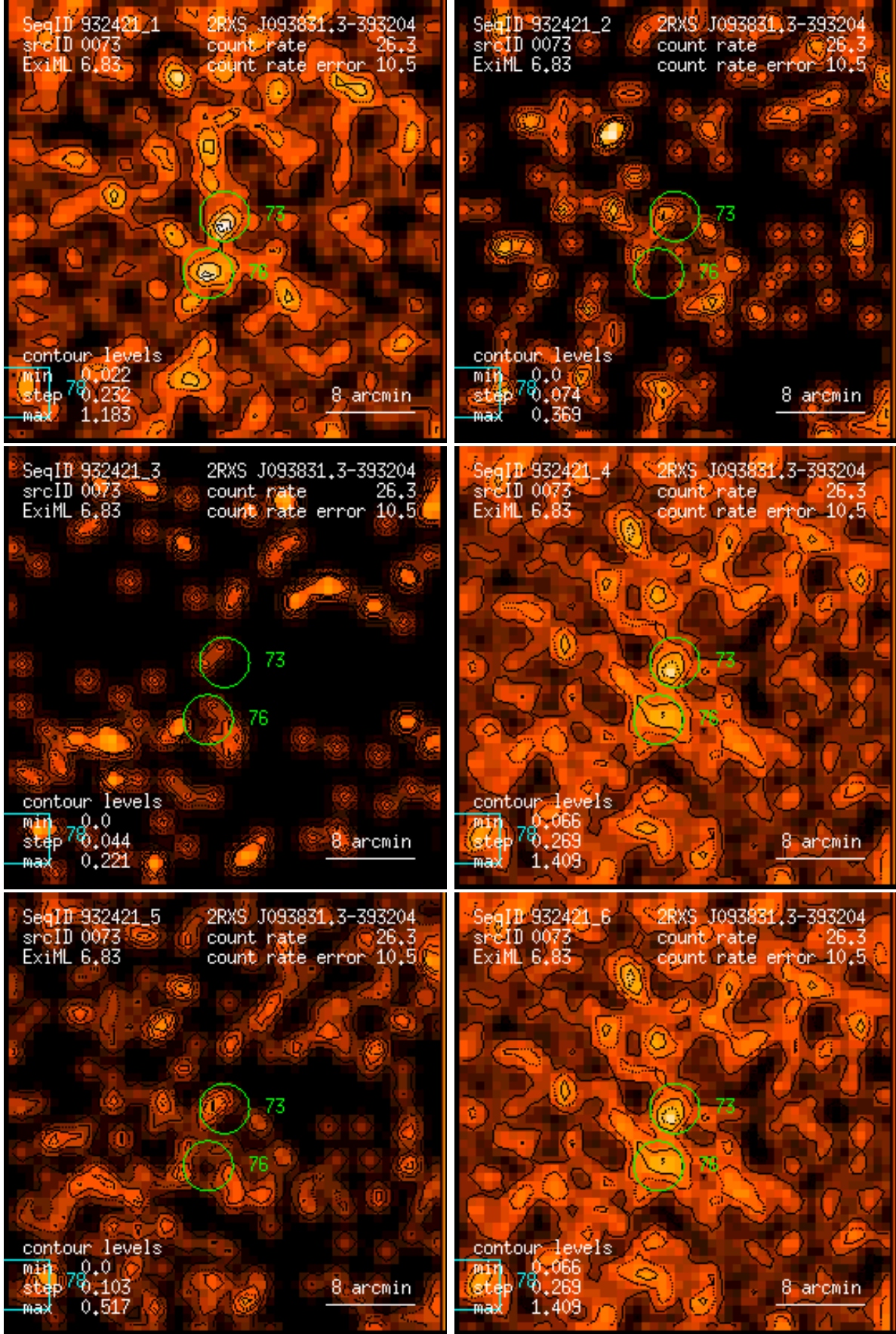
Figure 73: RASS 932421: detection 0073: band rate images, Gaussian filter: (1) PSPC channels 11 – 41, (2) 52 – 90, (3) 91 – 201, (4) 11 – 235, (5) 52 – 201, (6) 11 – 201. Broad band rates in counts/ks. Band rate contour levels in counts/ks/arcmin 2 .
