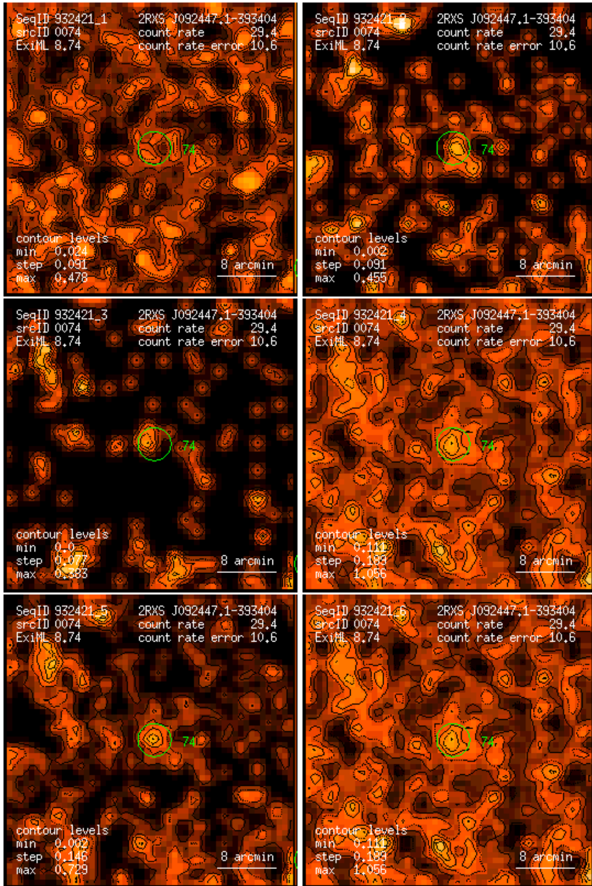
Figure 74: RASS 932421: detection 0074: band rate images, Gaussian filter: (1) PSPC channels 11 – 41, (2) 52 – 90, (3) 91 – 201, (4) 11 – 235, (5) 52 – 201, (6) 11 – 201. Broad band rates in counts/ks. Band rate contour levels in counts/ks/arcmin 2 .
