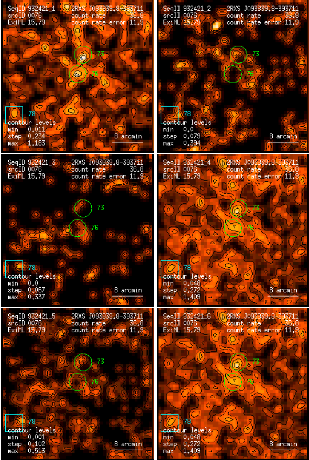
Figure 76: RASS 932421: detection 0076: band rate images, Gaussian filter: (1) PSPC channels 11 – 41, (2) 52 – 90, (3) 91 – 201, (4) 11 – 235, (5) 52 – 201, (6) 11 – 201. Broad band rates in counts/ks. Band rate contour levels in counts/ks/arcmin 2 .
