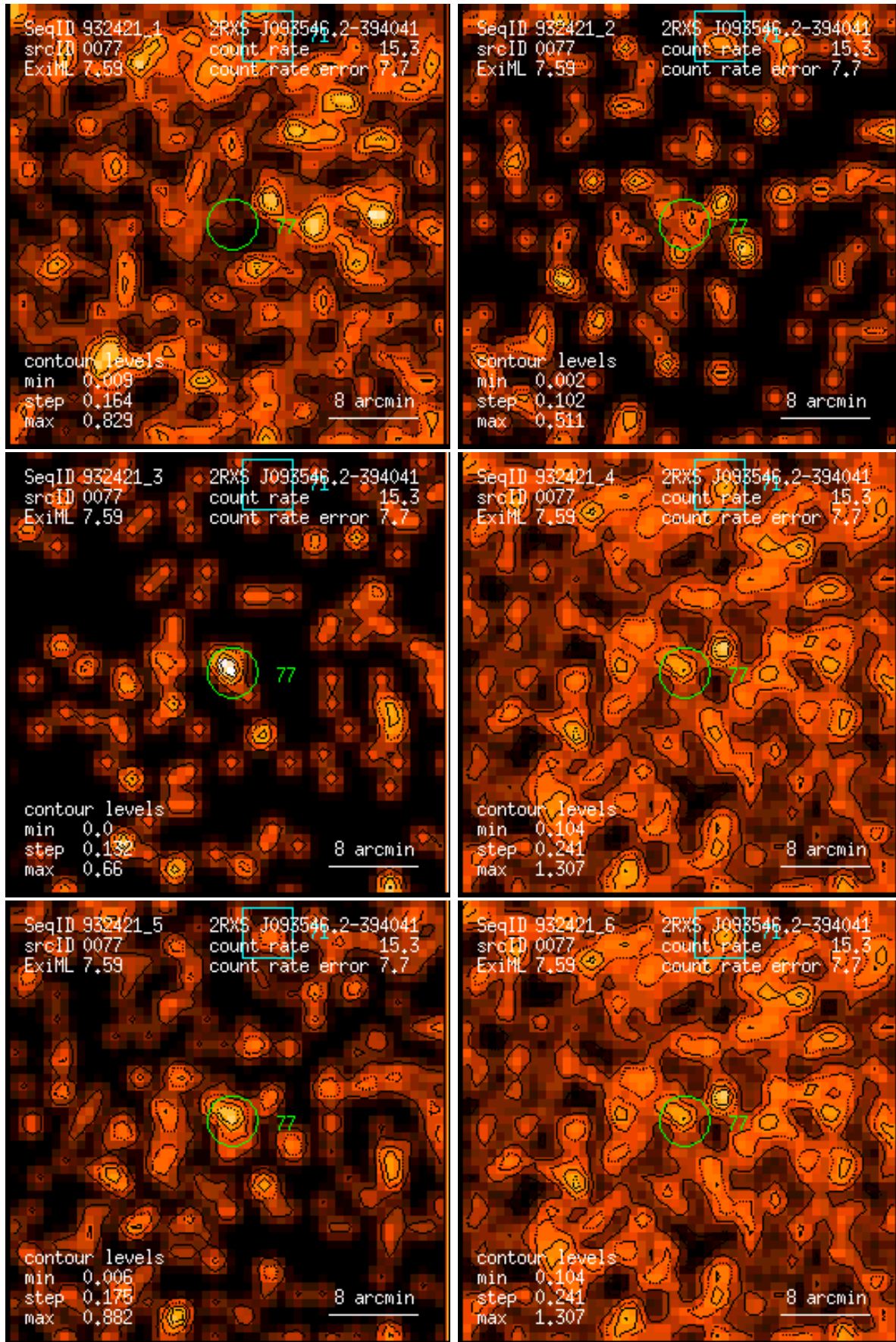
Figure 77: RASS 932421: detection 0077: band rate images, Gaussian filter: (1) PSPC channels 11 – 41, (2) 52 – 90, (3) 91 – 201, (4) 11 – 235, (5) 52 – 201, (6) 11 – 201. Broad band rates in counts/ks. Band rate contour levels in counts/ks/arcmin 2 .
