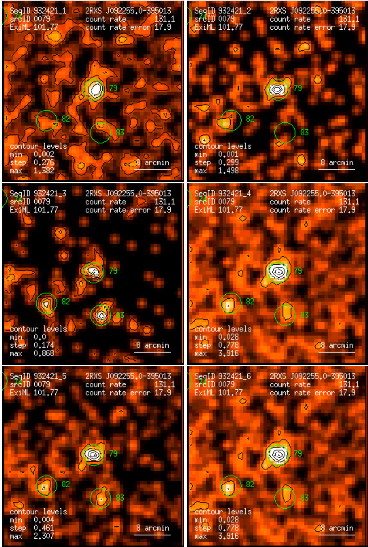
Figure 79: RASS 932421: detection 0079: band rate images, Gaussian filter: (1) PSPC channels 11 – 41, (2) 52 – 90, (3) 91 – 201, (4) 11 – 235, (5) 52 – 201, (6) 11 – 201. Broad band rates in counts/ks. Band rate contour levels in counts/ks/arcmin 2 .
