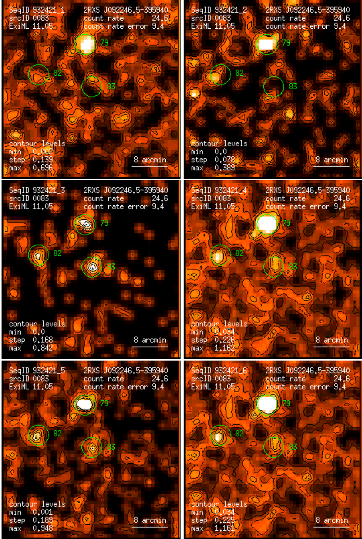
Figure 83: RASS 932421: detection 0083: band rate images, Gaussian filter: (1) PSPC channels 11 – 41, (2) 52 – 90, (3) 91 – 201, (4) 11 – 235, (5) 52 – 201, (6) 11 – 201. Broad band rates in counts/ks. Band rate contour levels in counts/ks/arcmin 2 .
