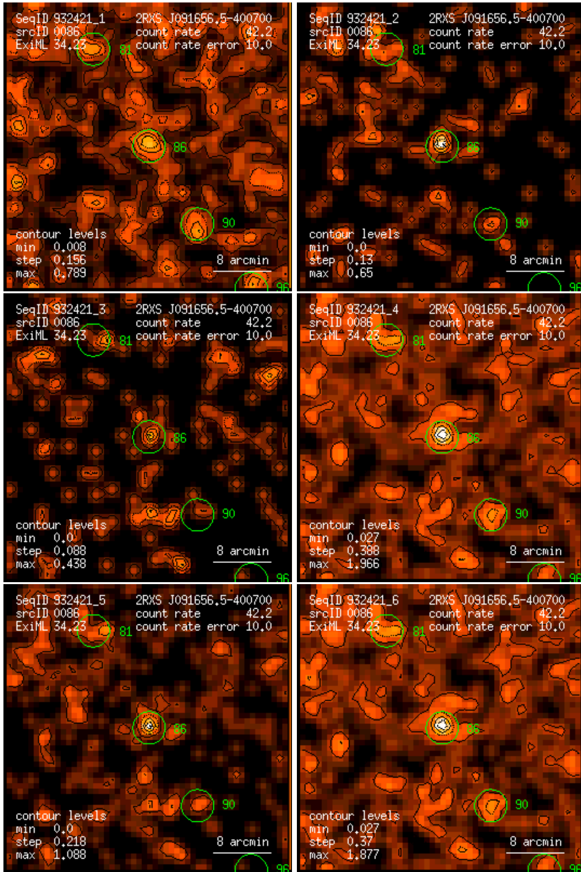
Figure 86: RASS 932421: detection 0086: band rate images, Gaussian filter: (1) PSPC channels 11 – 41, (2) 52 – 90, (3) 91 – 201, (4) 11 – 235, (5) 52 – 201, (6) 11 – 201. Broad band rates in counts/ks. Band rate contour levels in counts/ks/arcmin 2 .
