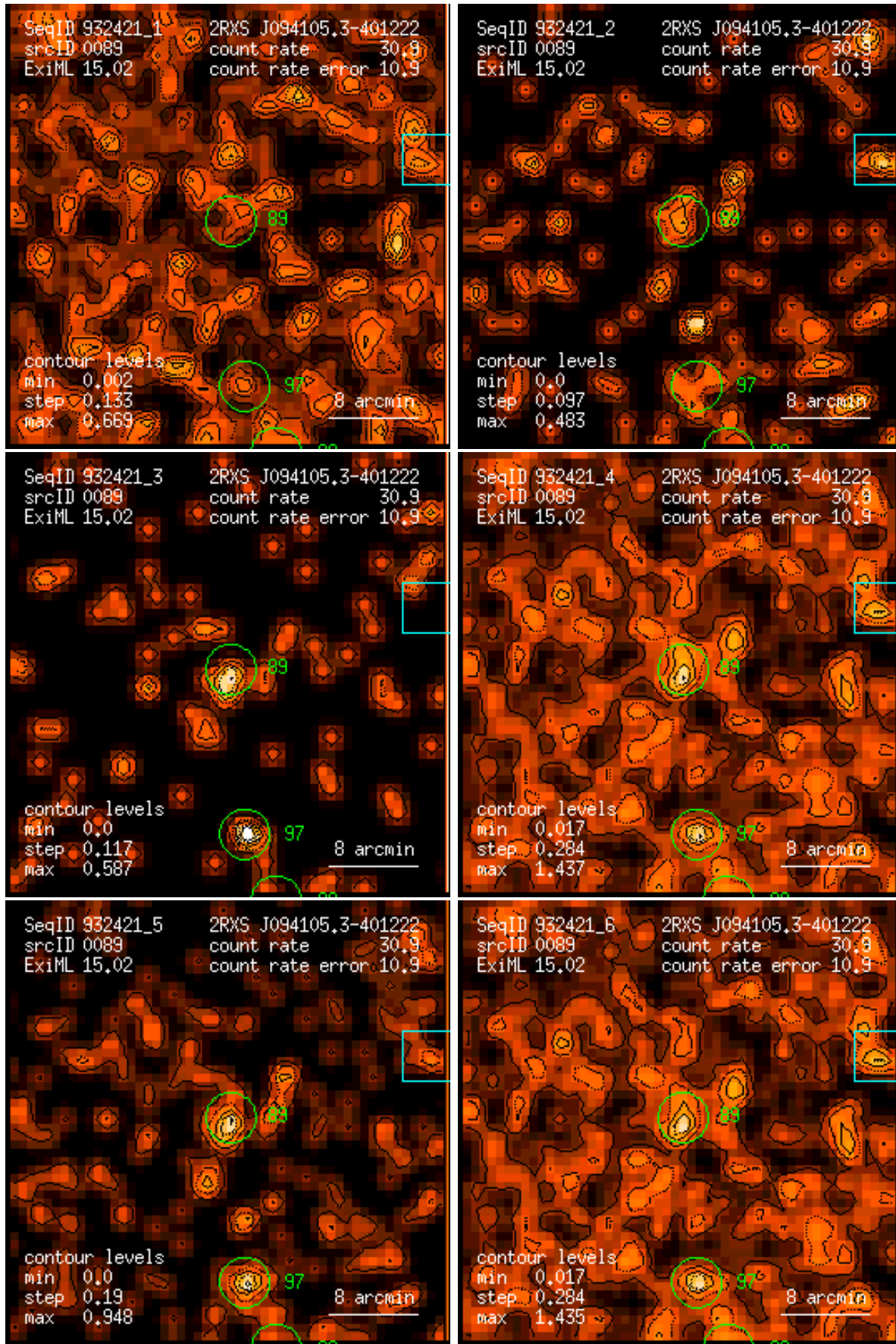
Figure 89: RASS 932421: detection 0089: band rate images, Gaussian filter: (1) PSPC channels 11 – 41, (2) 52 – 90, (3) 91 – 201, (4) 11 – 235, (5) 52 – 201, (6) 11 – 201. Broad band rates in counts/ks. Band rate contour levels in counts/ks/arcmin 2 .
