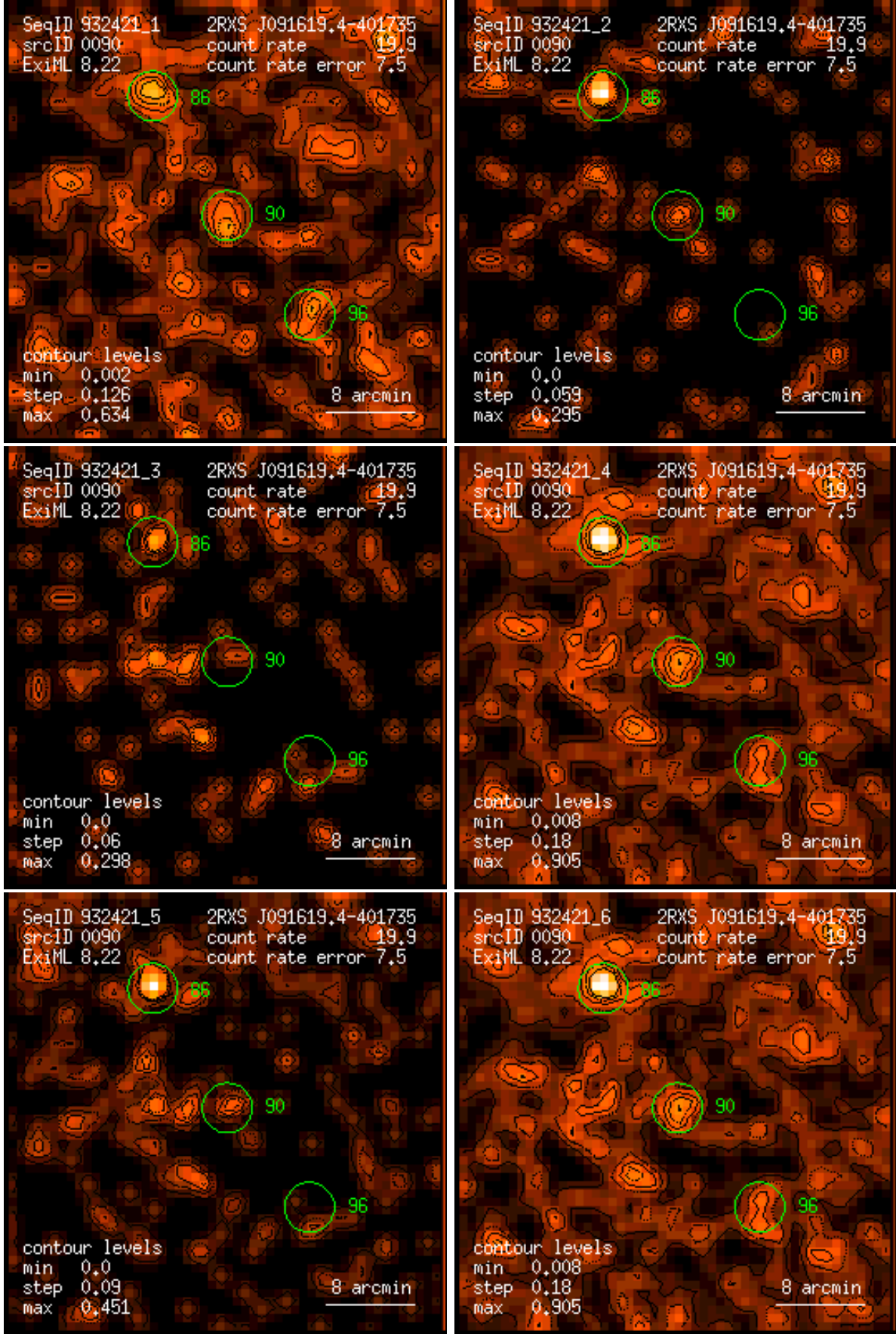
Figure 90: RASS 932421: detection 0090: band rate images, Gaussian filter: (1) PSPC channels 11 – 41, (2) 52 – 90, (3) 91 – 201, (4) 11 – 235, (5) 52 – 201, (6) 11 – 201. Broad band rates in counts/ks. Band rate contour levels in counts/ks/arcmin 2 .
