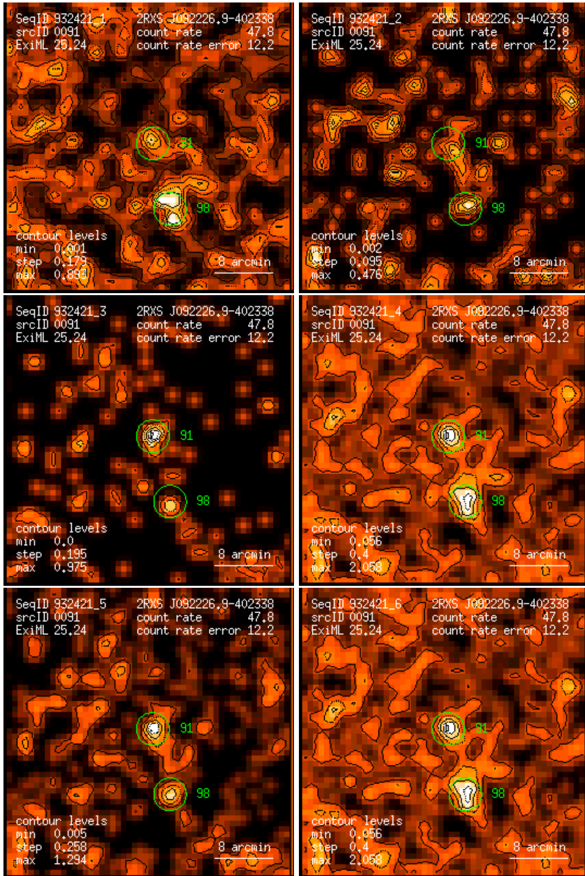
Figure 91: RASS 932421: detection 0091: band rate images, Gaussian filter: (1) PSPC channels 11 – 41, (2) 52 – 90, (3) 91 – 201, (4) 11 – 235, (5) 52 – 201, (6) 11 – 201. Broad band rates in counts/ks. Band rate contour levels in counts/ks/arcmin 2 .
