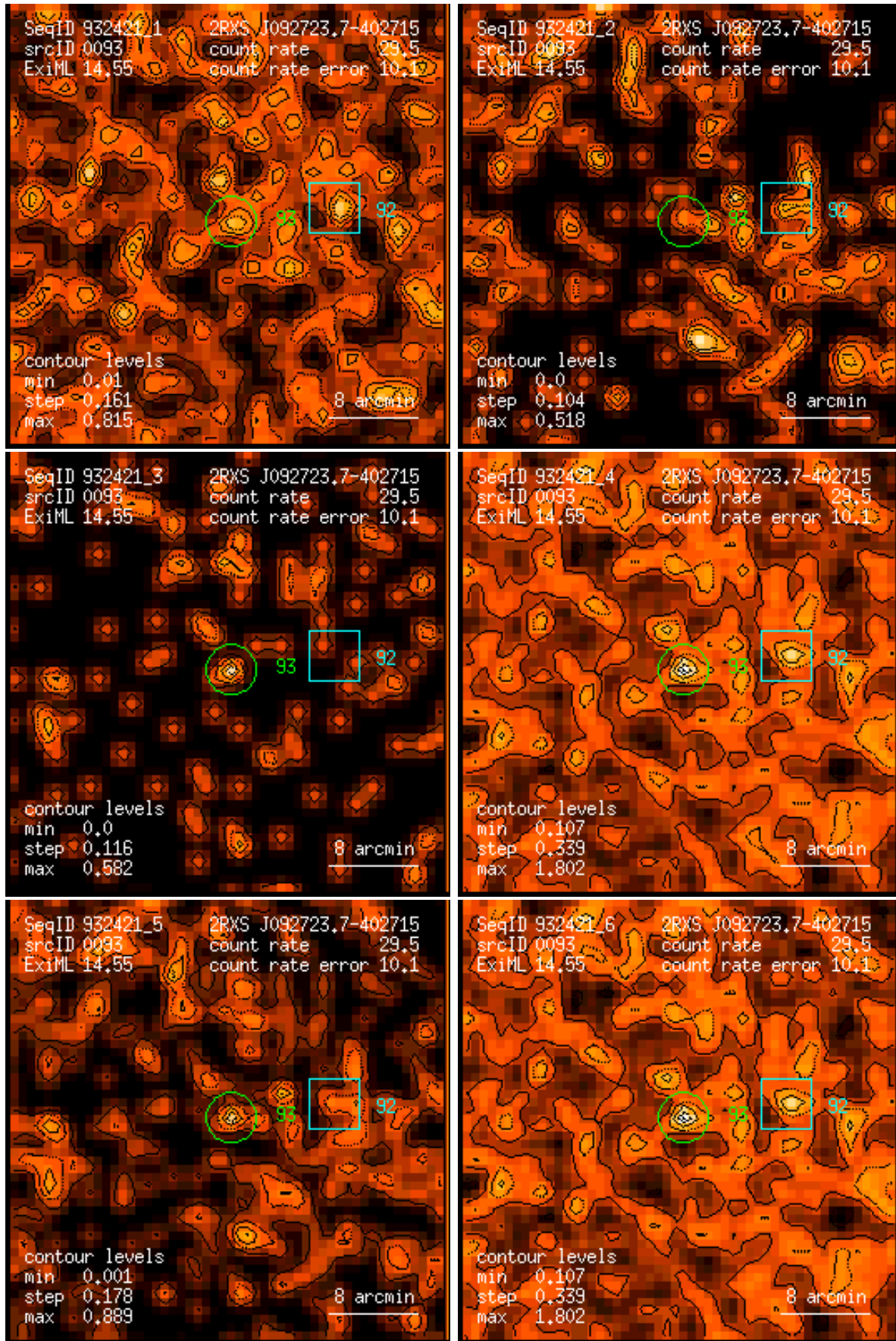
Figure 93: RASS 932421: detection 0093: band rate images, Gaussian filter: (1) PSPC channels 11 – 41, (2) 52 – 90, (3) 91 – 201, (4) 11 – 235, (5) 52 – 201, (6) 11 – 201. Broad band rates in counts/ks. Band rate contour levels in counts/ks/arcmin 2 .
