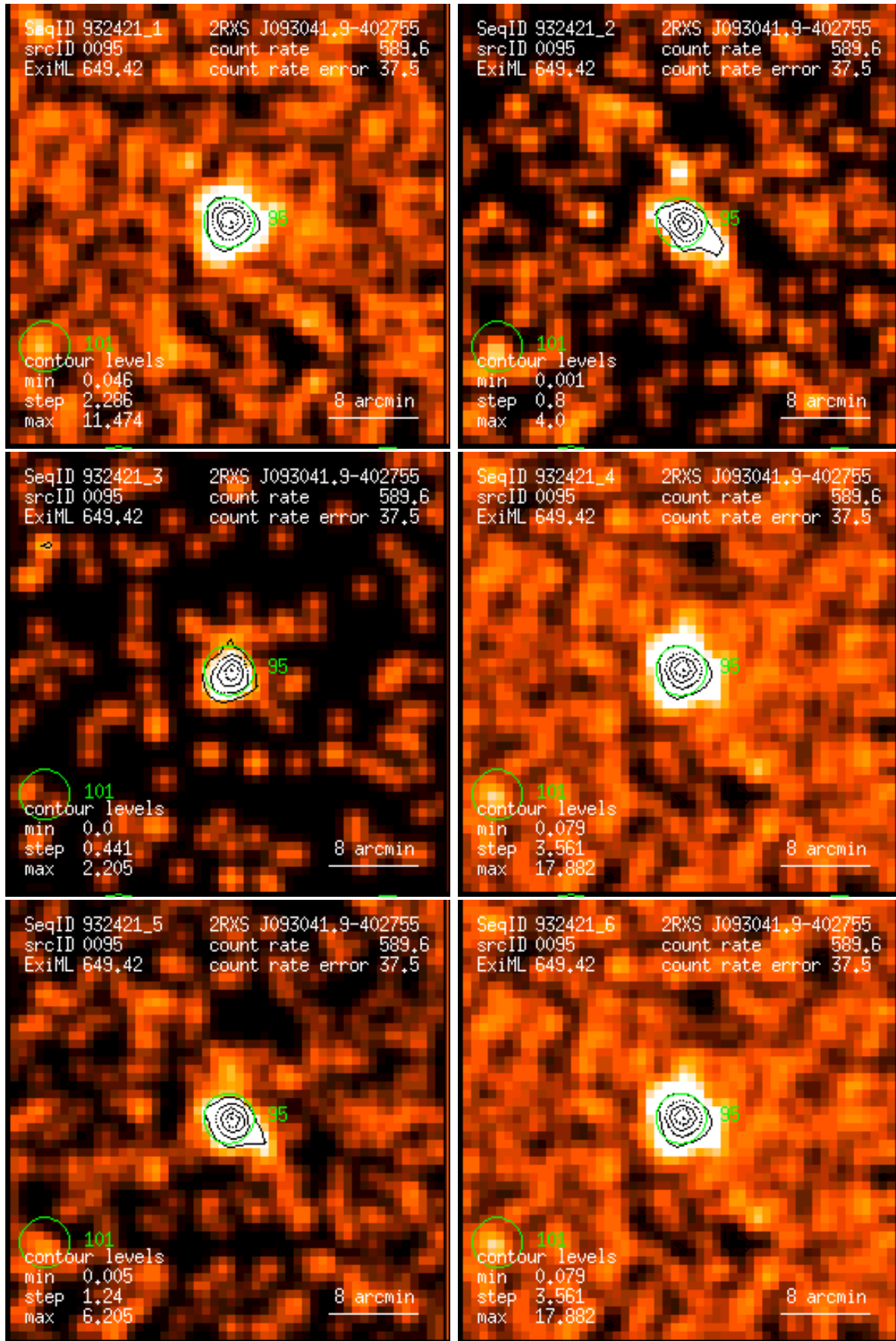
Figure 95: RASS 932421: detection 0095: band rate images, Gaussian filter: (1) PSPC channels 11 – 41, (2) 52 – 90, (3) 91 – 201, (4) 11 – 235, (5) 52 – 201, (6) 11 – 201. Broad band rates in counts/ks. Band rate contour levels in counts/ks/arcmin 2 .
