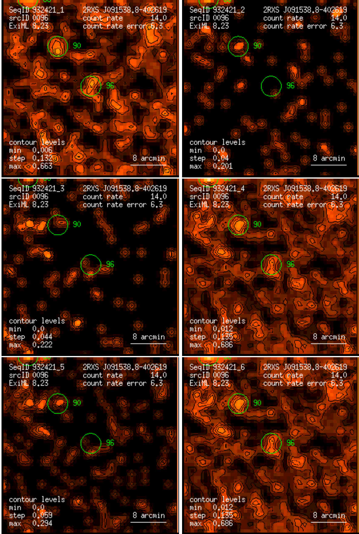
Figure 96: RASS 932421: detection 0096: band rate images, Gaussian filter: (1) PSPC channels 11 – 41, (2) 52 – 90, (3) 91 – 201, (4) 11 – 235, (5) 52 – 201, (6) 11 – 201. Broad band rates in counts/ks. Band rate contour levels in counts/ks/arcmin 2 .
