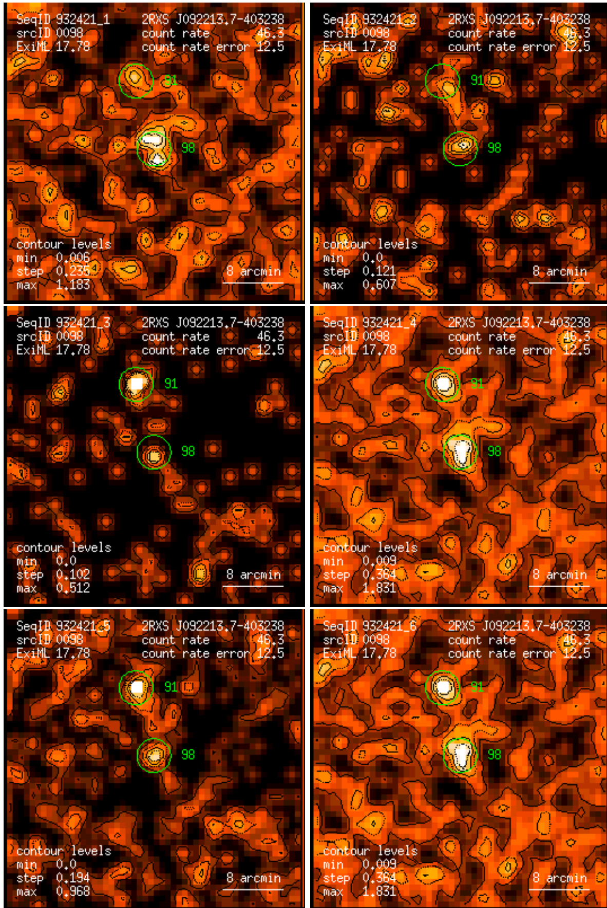
Figure 98: RASS 932421: detection 0098: band rate images, Gaussian filter: (1) PSPC channels 11 – 41, (2) 52 – 90, (3) 91 – 201, (4) 11 – 235, (5) 52 – 201, (6) 11 – 201. Broad band rates in counts/ks. Band rate contour levels in counts/ks/arcmin 2 .
