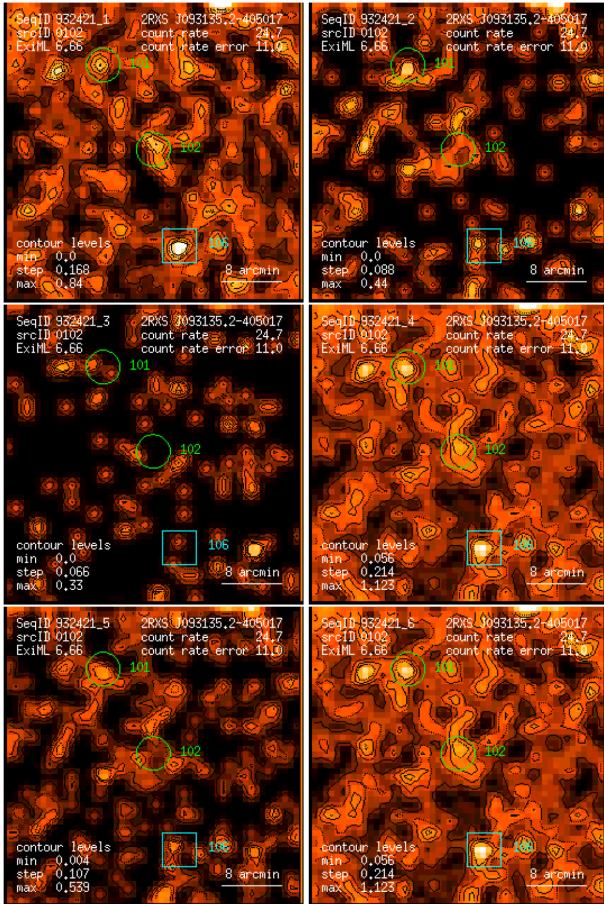
Figure 102: RASS 932421: detection 0102: band rate images, Gaussian filter: (1) PSPC channels 11 – 41, (2) 52 – 90, (3) 91 – 201, (4) 11 – 235, (5) 52 – 201, (6) 11 – 201. Broad band rates in counts/ks. Band rate contour levels in counts/ks/arcmin 2 .
