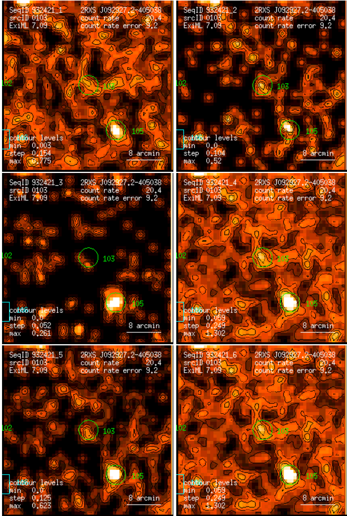
Figure 103: RASS 932421: detection 0103: band rate images, Gaussian filter: (1) PSPC channels 11 – 41, (2) 52 – 90, (3) 91 – 201, (4) 11 – 235, (5) 52 – 201, (6) 11 – 201. Broad band rates in counts/ks. Band rate contour levels in counts/ks/arcmin 2 .
