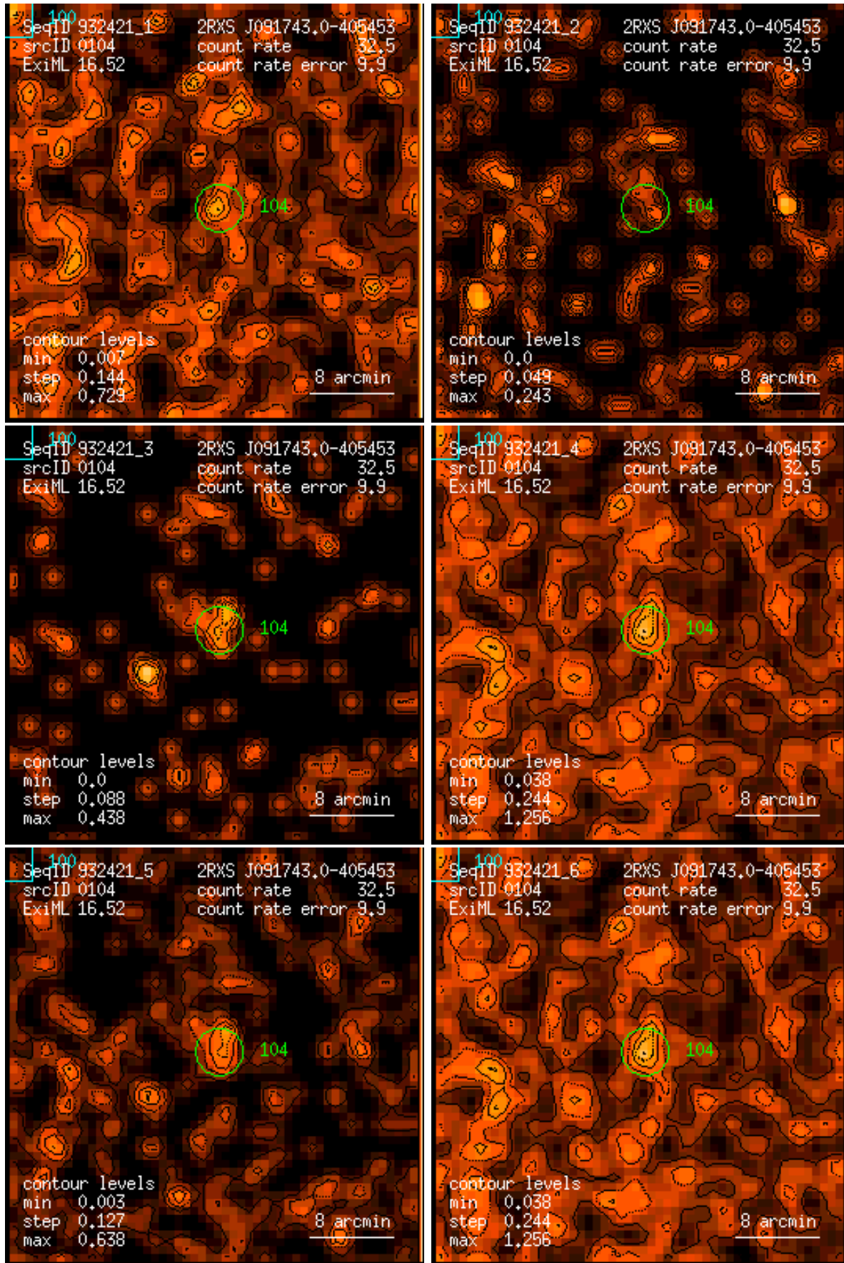
Figure 104: RASS 932421: detection 0104: band rate images, Gaussian filter: (1) PSPC channels 11 – 41, (2) 52 – 90, (3) 91 – 201, (4) 11 – 235, (5) 52 – 201, (6) 11 – 201. Broad band rates in counts/ks. Band rate contour levels in counts/ks/arcmin 2 .
