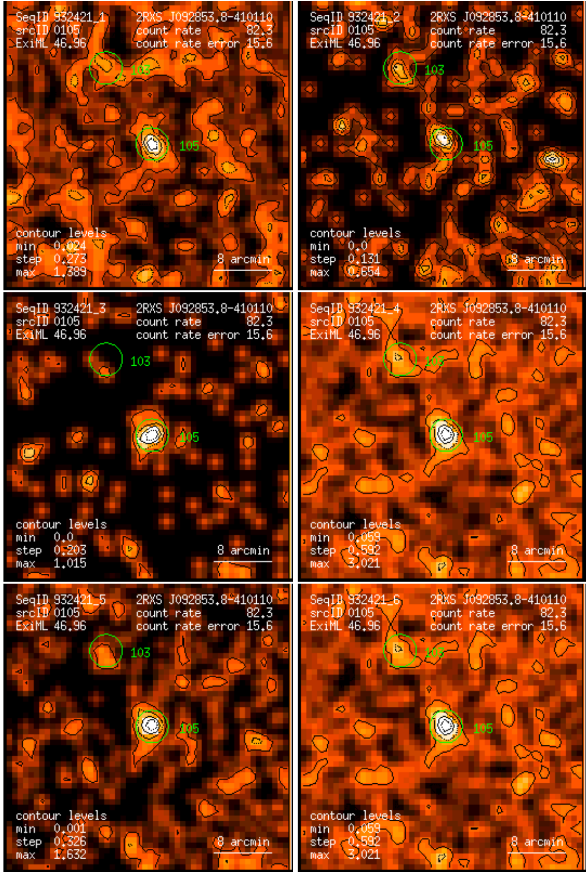
Figure 105: RASS 932421: detection 0105: band rate images, Gaussian filter: (1) PSPC channels 11 – 41, (2) 52 – 90, (3) 91 – 201, (4) 11 – 235, (5) 52 – 201, (6) 11 – 201. Broad band rates in counts/ks. Band rate contour levels in counts/ks/arcmin 2 .
