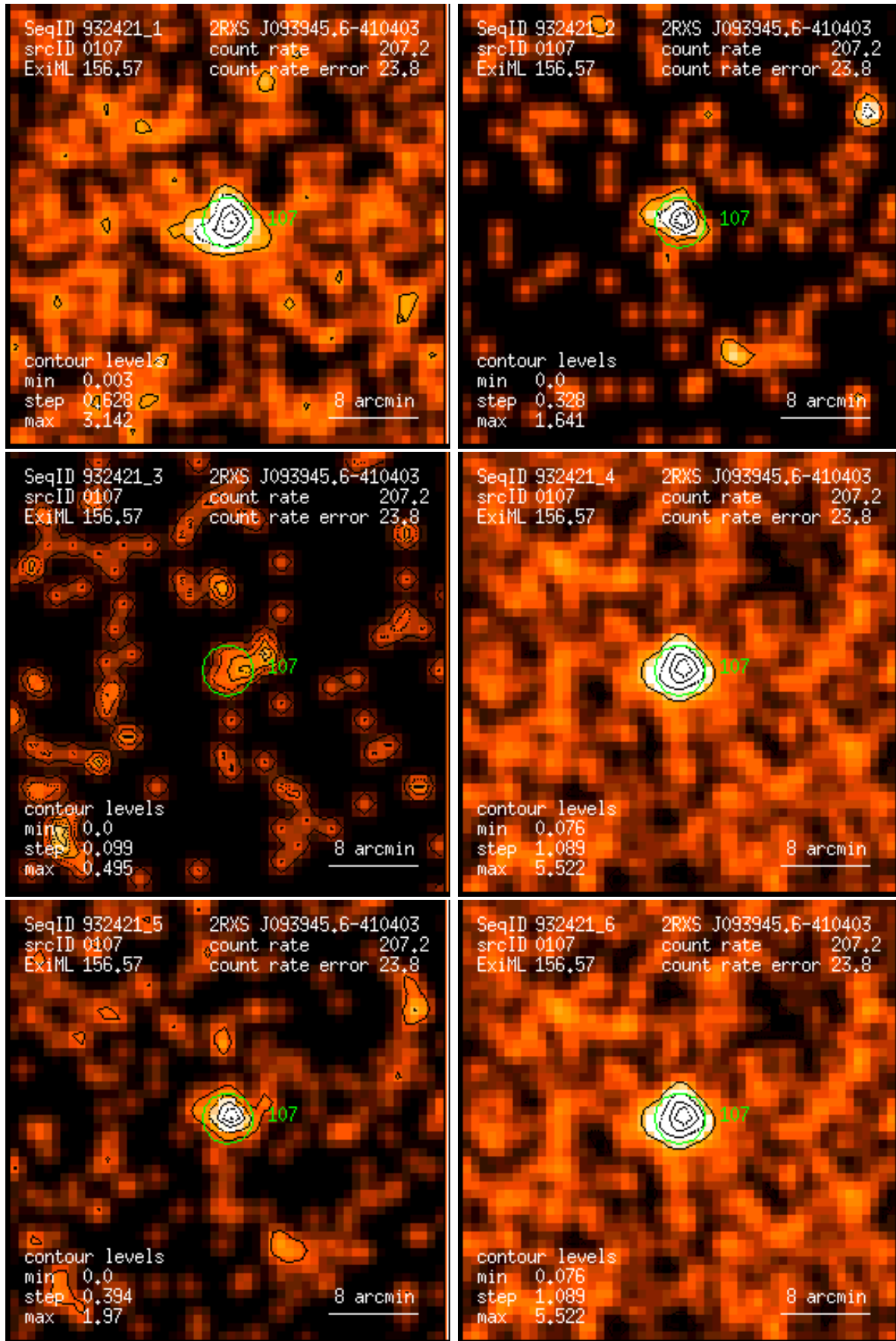
Figure 107: RASS 932421: detection 0107: band rate images, Gaussian filter: (1) PSPC channels 11 – 41, (2) 52 – 90, (3) 91 – 201, (4) 11 – 235, (5) 52 – 201, (6) 11 – 201. Broad band rates in counts/ks. Band rate contour levels in counts/ks/arcmin 2 .
