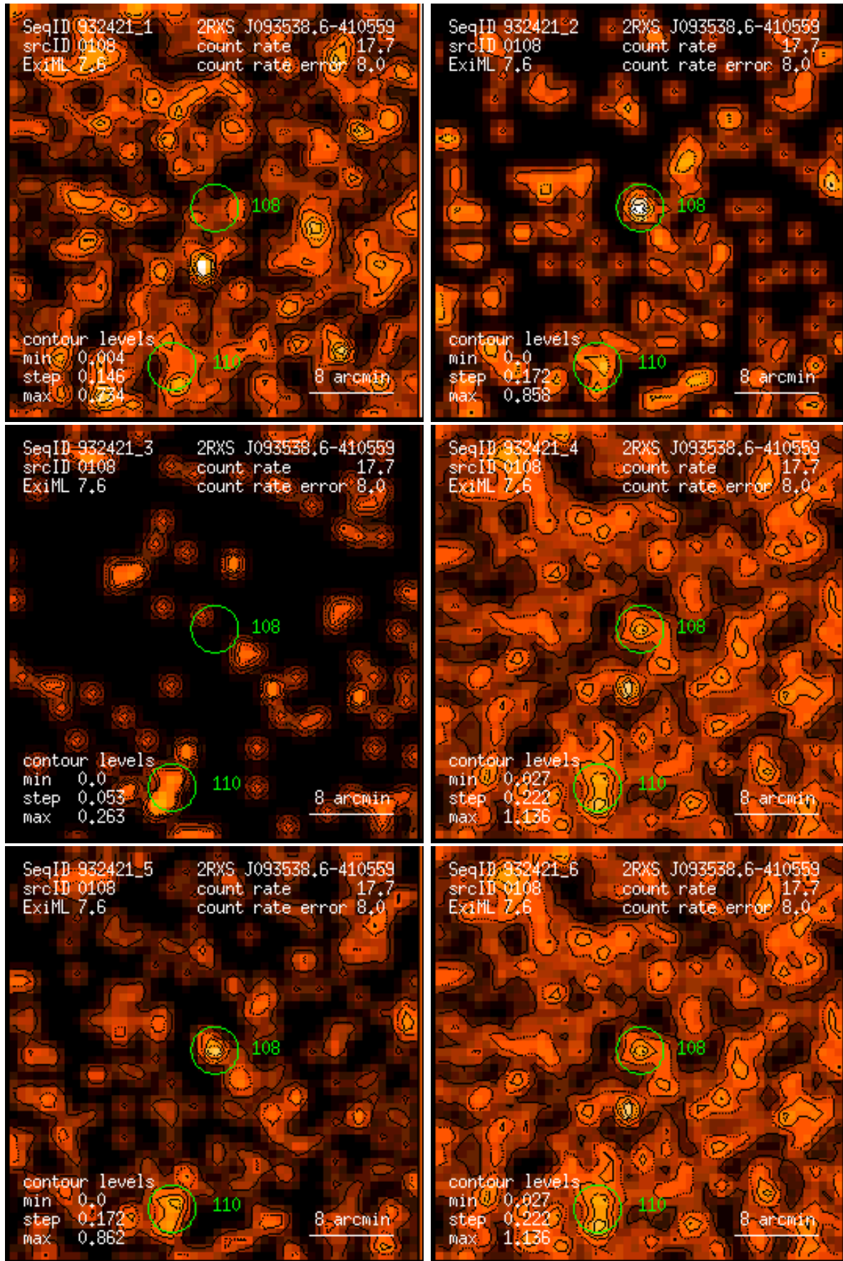
Figure 108: RASS 932421: detection 0108: band rate images, Gaussian filter: (1) PSPC channels 11 – 41, (2) 52 – 90, (3) 91 – 201, (4) 11 – 235, (5) 52 – 201, (6) 11 – 201. Broad band rates in counts/ks. Band rate contour levels in counts/ks/arcmin 2 .
