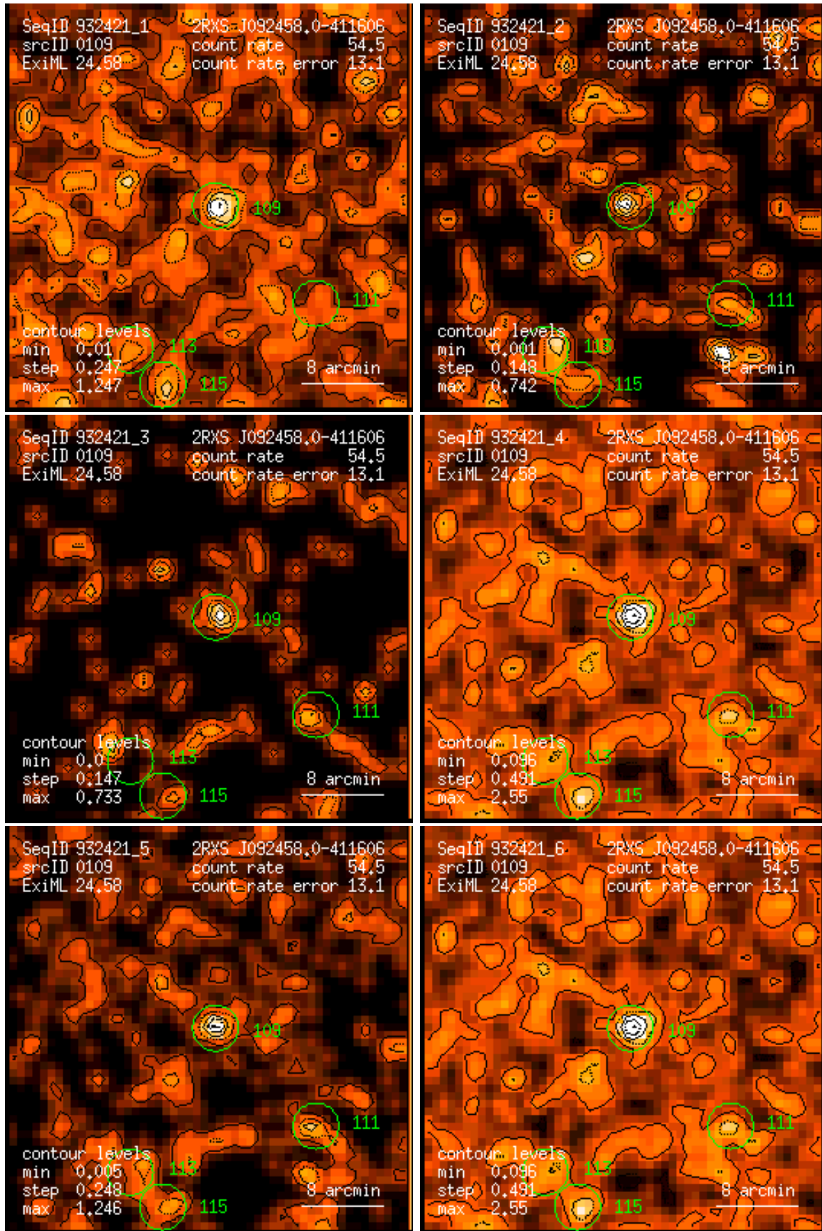
Figure 109: RASS 932421: detection 0109: band rate images, Gaussian filter: (1) PSPC channels 11 – 41, (2) 52 – 90, (3) 91 – 201, (4) 11 – 235, (5) 52 – 201, (6) 11 – 201. Broad band rates in counts/ks. Band rate contour levels in counts/ks/arcmin 2 .
