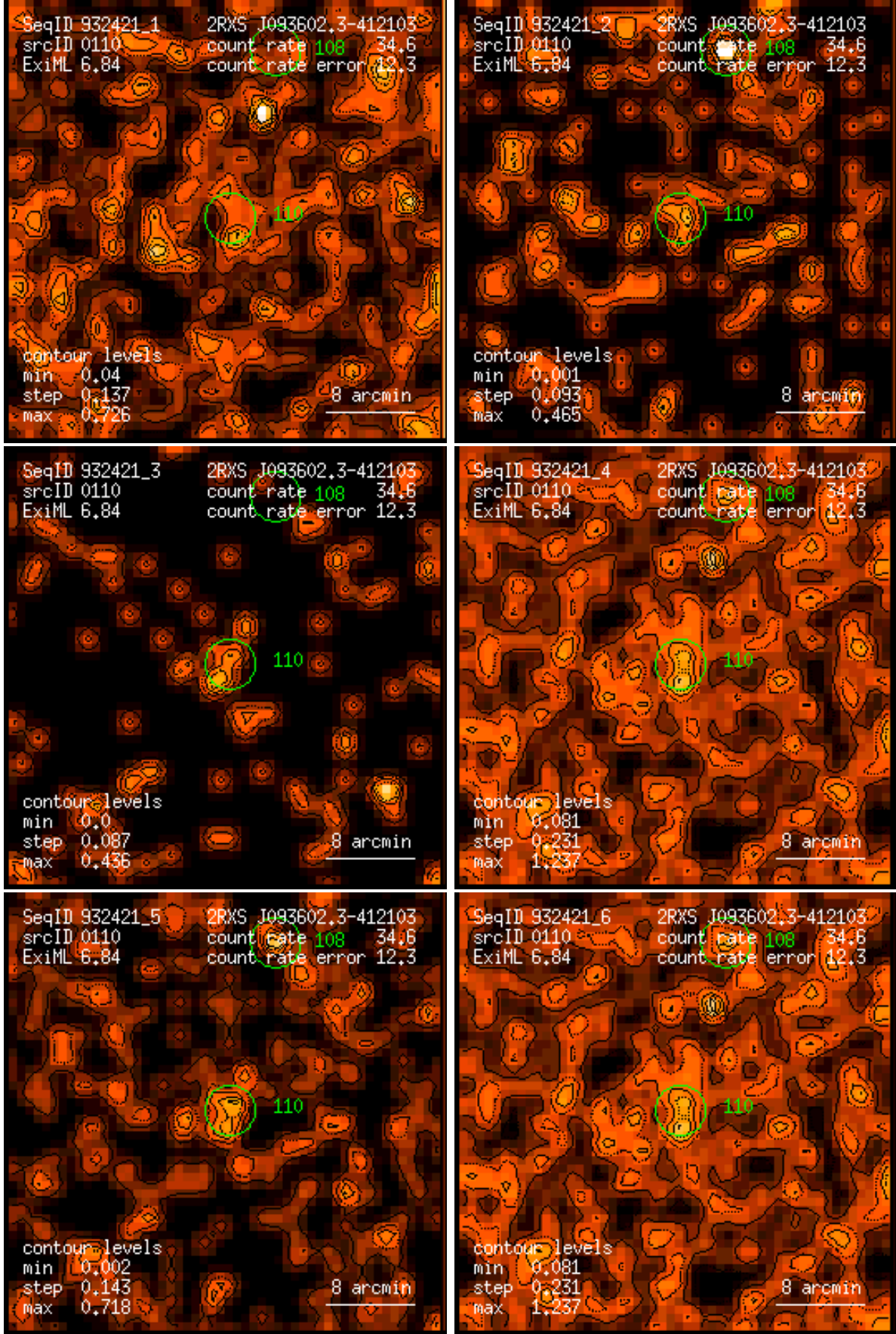
Figure 110: RASS 932421: detection 0110: band rate images, Gaussian filter: (1) PSPC channels 11 – 41, (2) 52 – 90, (3) 91 – 201, (4) 11 – 235, (5) 52 – 201, (6) 11 – 201. Broad band rates in counts/ks. Band rate contour levels in counts/ks/arcmin 2 .
