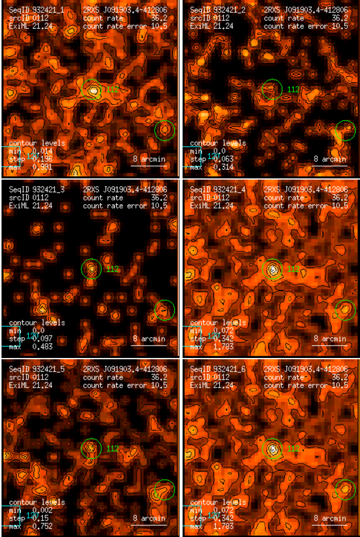
Figure 112: RASS 932421: detection 0112: band rate images, Gaussian filter: (1) PSPC channels 11 – 41, (2) 52 – 90, (3) 91 – 201, (4) 11 – 235, (5) 52 – 201, (6) 11 – 201. Broad band rates in counts/ks. Band rate contour levels in counts/ks/arcmin 2 .
