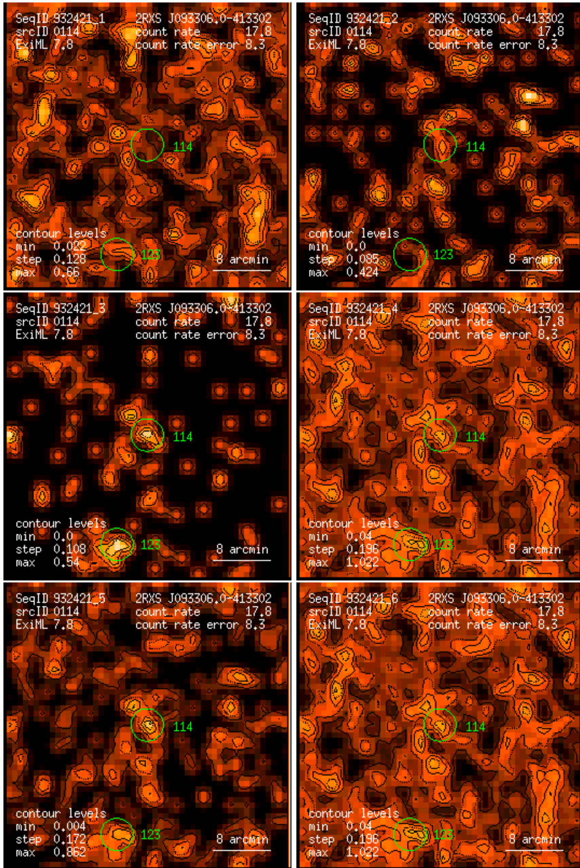
Figure 114: RASS 932421: detection 0114: band rate images, Gaussian filter: (1) PSPC channels 11 – 41, (2) 52 – 90, (3) 91 – 201, (4) 11 – 235, (5) 52 – 201, (6) 11 – 201. Broad band rates in counts/ks. Band rate contour levels in counts/ks/arcmin 2 .
