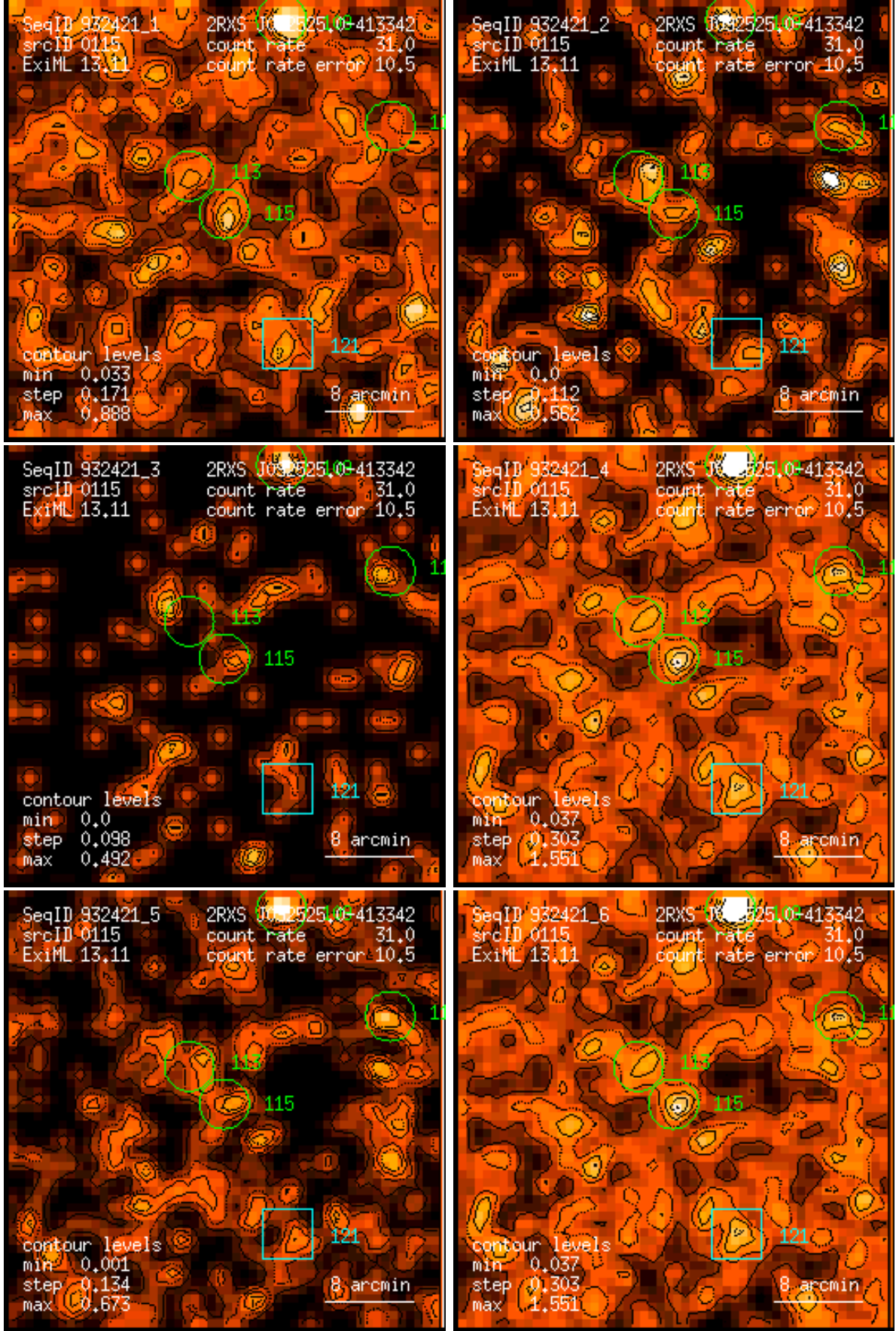
Figure 115: RASS 932421: detection 0115: band rate images, Gaussian filter: (1) PSPC channels 11 – 41, (2) 52 – 90, (3) 91 – 201, (4) 11 – 235, (5) 52 – 201, (6) 11 – 201. Broad band rates in counts/ks. Band rate contour levels in counts/ks/arcmin 2 .
