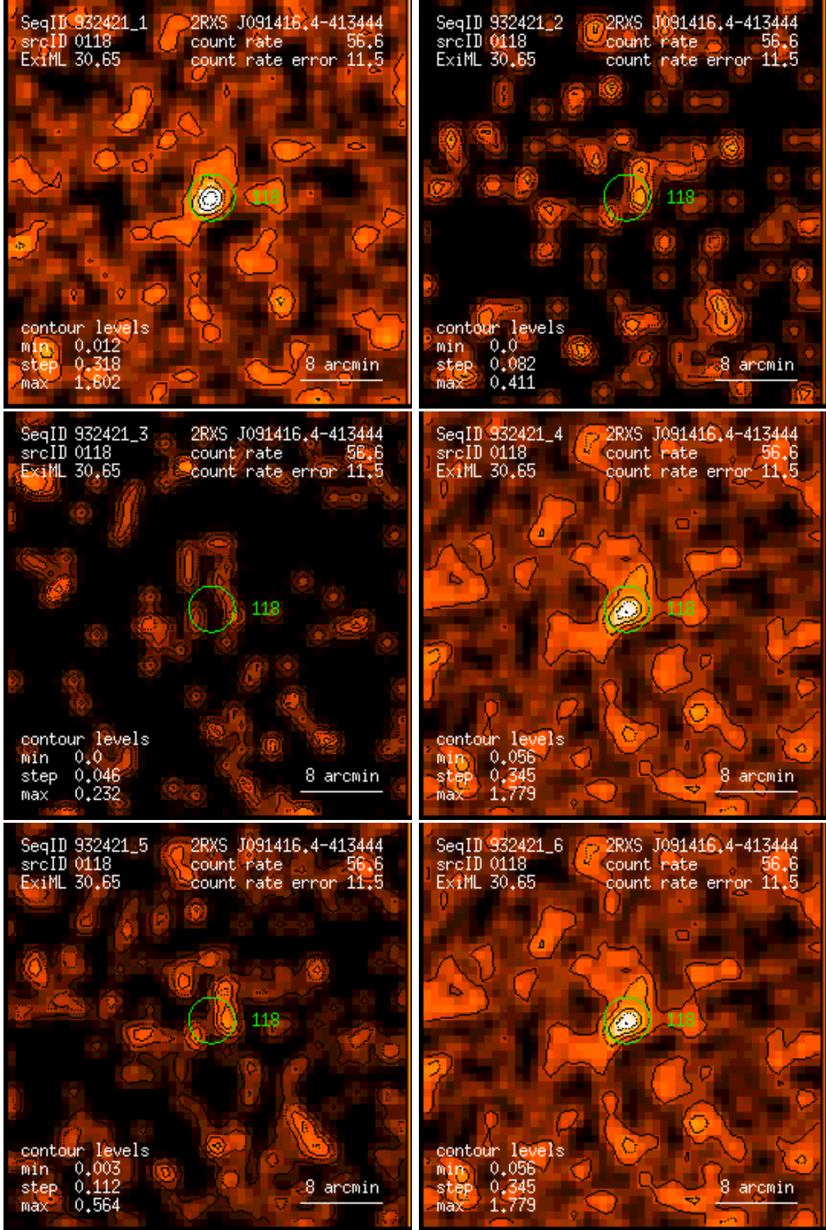
Figure 118: RASS 932421: detection 0118: band rate images, Gaussian filter: (1) PSPC channels 11 – 41, (2) 52 – 90, (3) 91 – 201, (4) 11 – 235, (5) 52 – 201, (6) 11 – 201. Broad band rates in counts/ks. Band rate contour levels in counts/ks/arcmin 2 .
