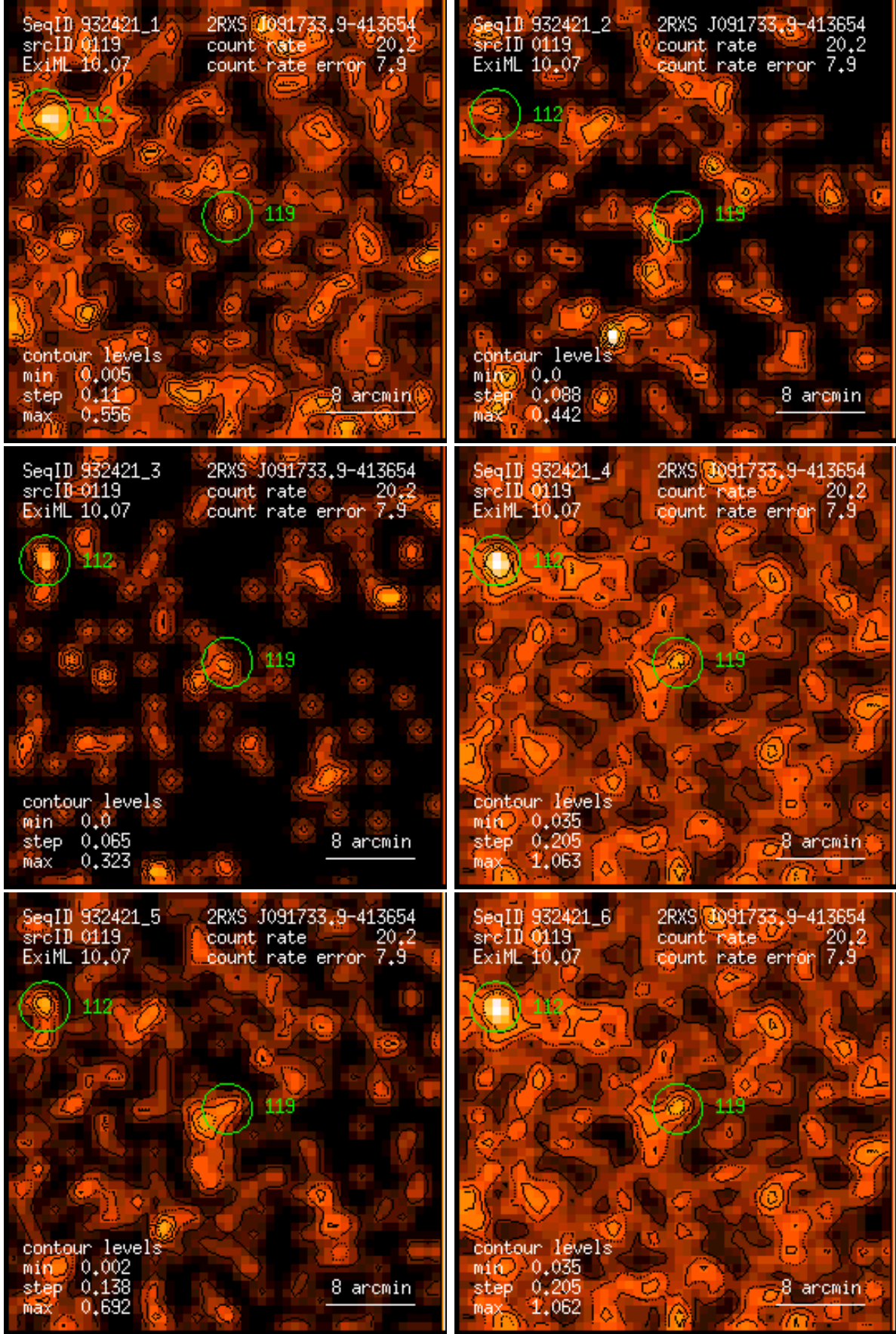
Figure 119: RASS 932421: detection 0119: band rate images, Gaussian filter: (1) PSPC channels 11 – 41, (2) 52 – 90, (3) 91 – 201, (4) 11 – 235, (5) 52 – 201, (6) 11 – 201. Broad band rates in counts/ks. Band rate contour levels in counts/ks/arcmin 2 .
