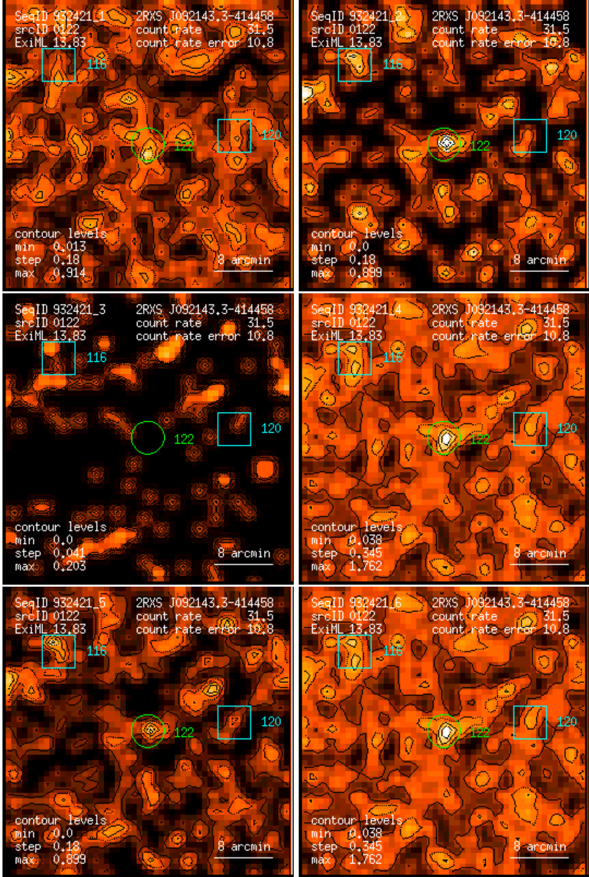
Figure 122: RASS 932421: detection 0122: band rate images, Gaussian filter: (1) PSPC channels 11 – 41, (2) 52 – 90, (3) 91 – 201, (4) 11 – 235, (5) 52 – 201, (6) 11 – 201. Broad band rates in counts/ks. Band rate contour levels in counts/ks/arcmin 2 .
