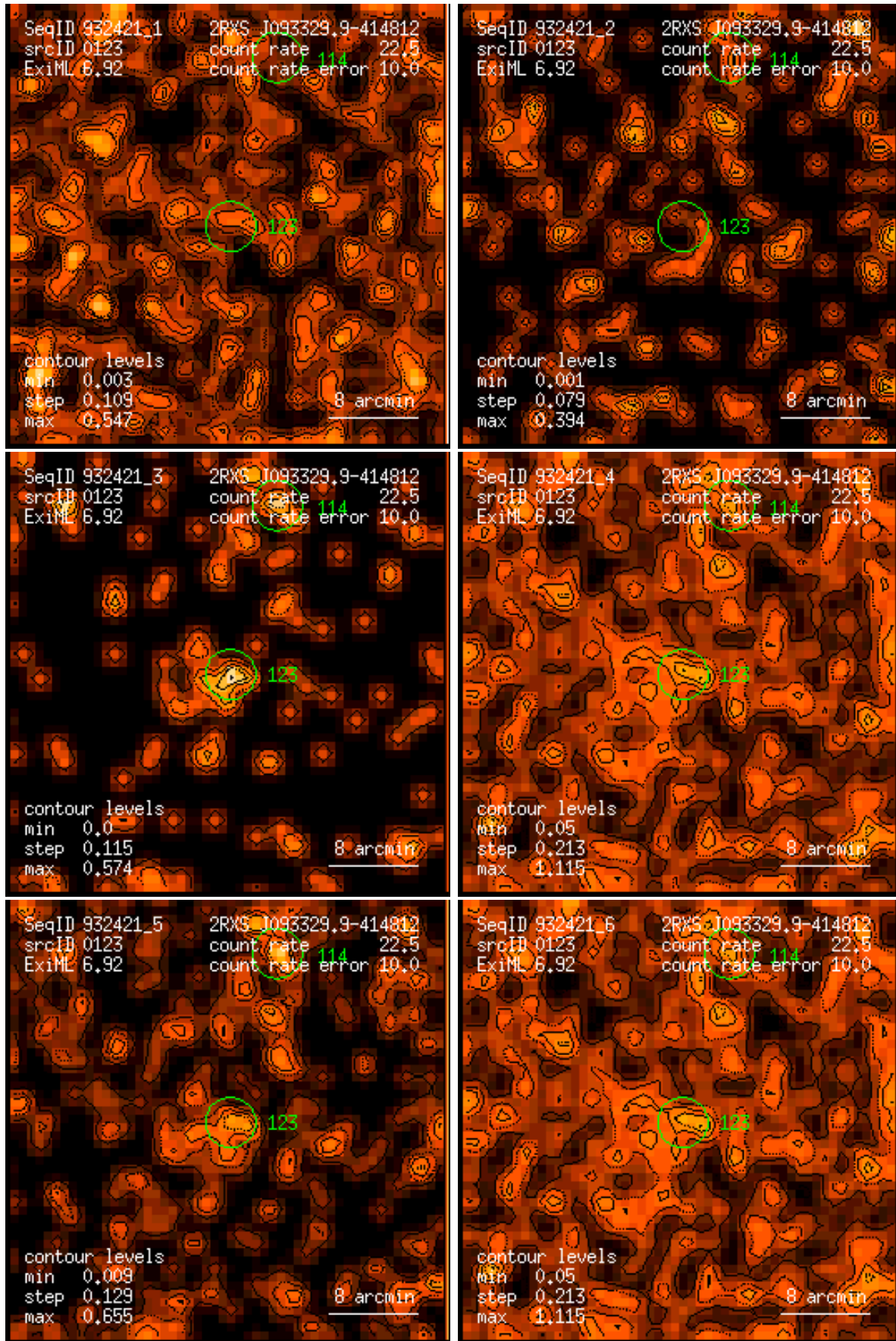
Figure 123: RASS 932421: detection 0123: band rate images, Gaussian filter: (1) PSPC channels 11 – 41, (2) 52 – 90, (3) 91 – 201, (4) 11 – 235, (5) 52 – 201, (6) 11 – 201. Broad band rates in counts/ks. Band rate contour levels in counts/ks/arcmin 2 .
