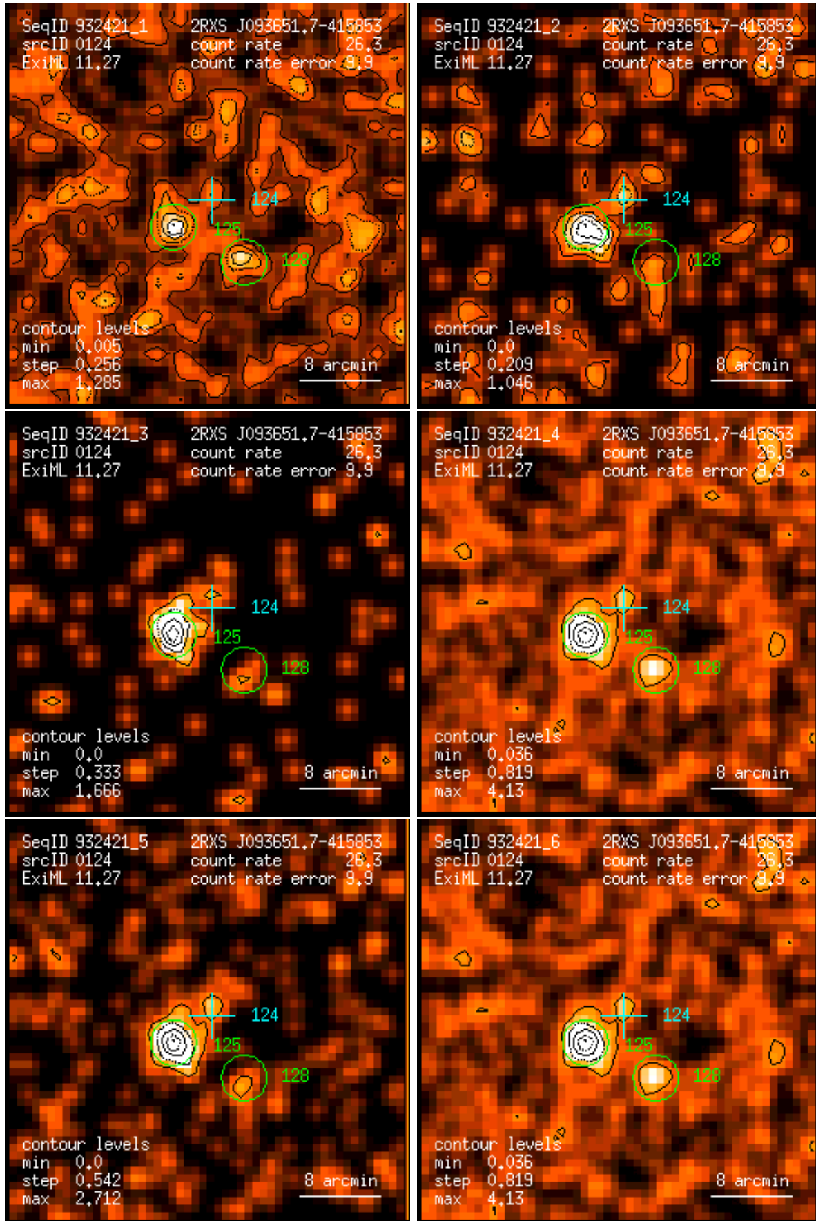
Figure 124: RASS 932421: detection 0124: band rate images, Gaussian filter: (1) PSPC channels 11 – 41, (2) 52 – 90, (3) 91 – 201, (4) 11 – 235, (5) 52 – 201, (6) 11 – 201. Broad band rates in counts/ks. Band rate contour levels in counts/ks/arcmin 2 .
