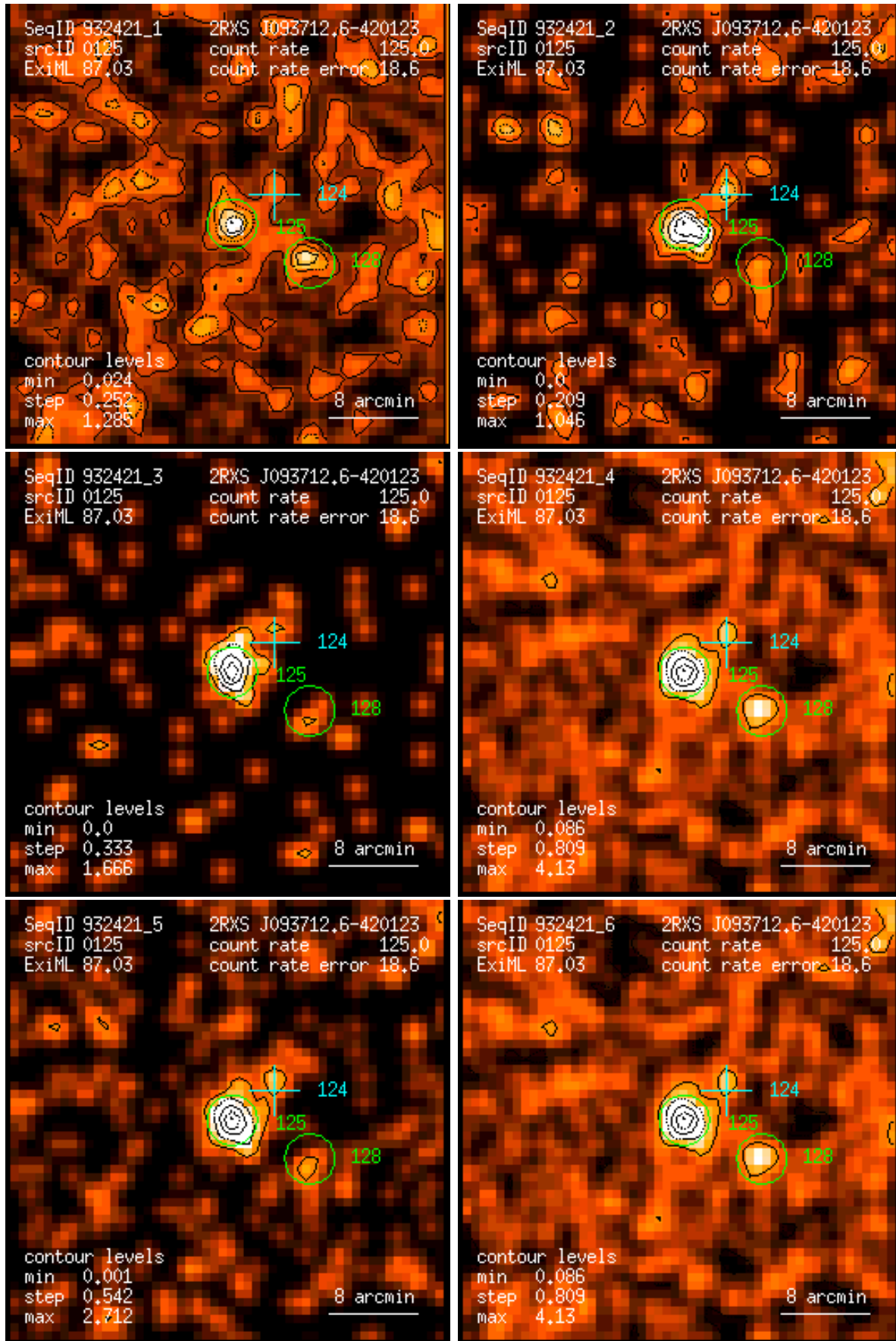
Figure 125: RASS 932421: detection 0125: band rate images, Gaussian filter: (1) PSPC channels 11 – 41, (2) 52 – 90, (3) 91 – 201, (4) 11 – 235, (5) 52 – 201, (6) 11 – 201. Broad band rates in counts/ks. Band rate contour levels in counts/ks/arcmin 2 .
