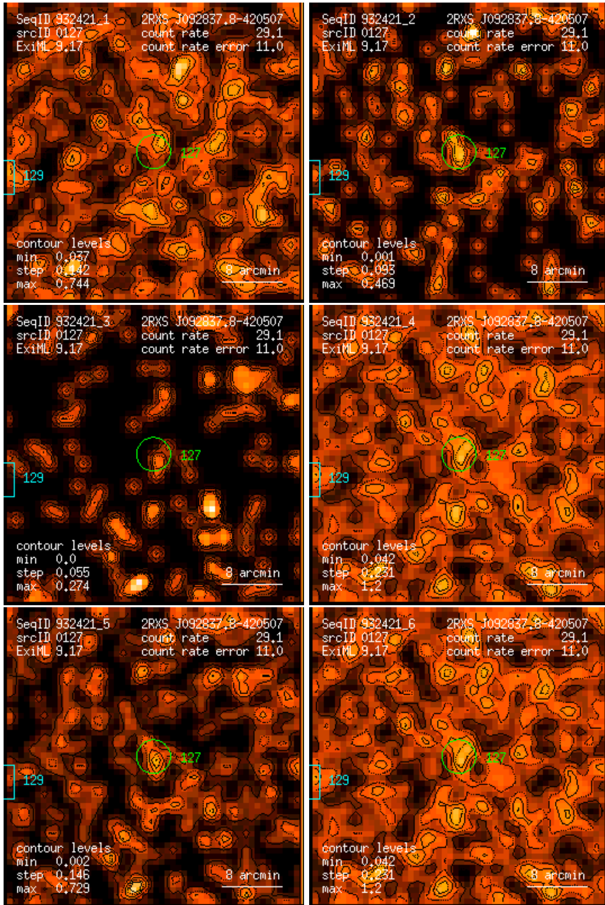
Figure 127: RASS 932421: detection 0127: band rate images, Gaussian filter: (1) PSPC channels 11 – 41, (2) 52 – 90, (3) 91 – 201, (4) 11 – 235, (5) 52 – 201, (6) 11 – 201. Broad band rates in counts/ks. Band rate contour levels in counts/ks/arcmin 2 .
