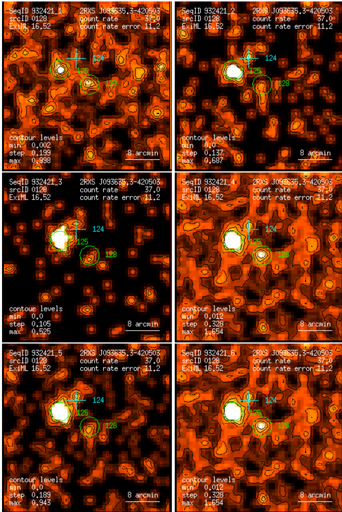
Figure 128: RASS 932421: detection 0128: band rate images, Gaussian filter: (1) PSPC channels 11 – 41, (2) 52 – 90, (3) 91 – 201, (4) 11 – 235, (5) 52 – 201, (6) 11 – 201. Broad band rates in counts/ks. Band rate contour levels in counts/ks/arcmin 2 .
