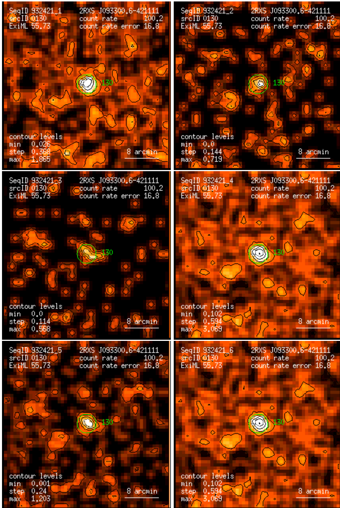
Figure 130: RASS 932421: detection 0130: band rate images, Gaussian filter: (1) PSPC channels 11 – 41, (2) 52 – 90, (3) 91 – 201, (4) 11 – 235, (5) 52 – 201, (6) 11 – 201. Broad band rates in counts/ks. Band rate contour levels in counts/ks/arcmin 2 .
