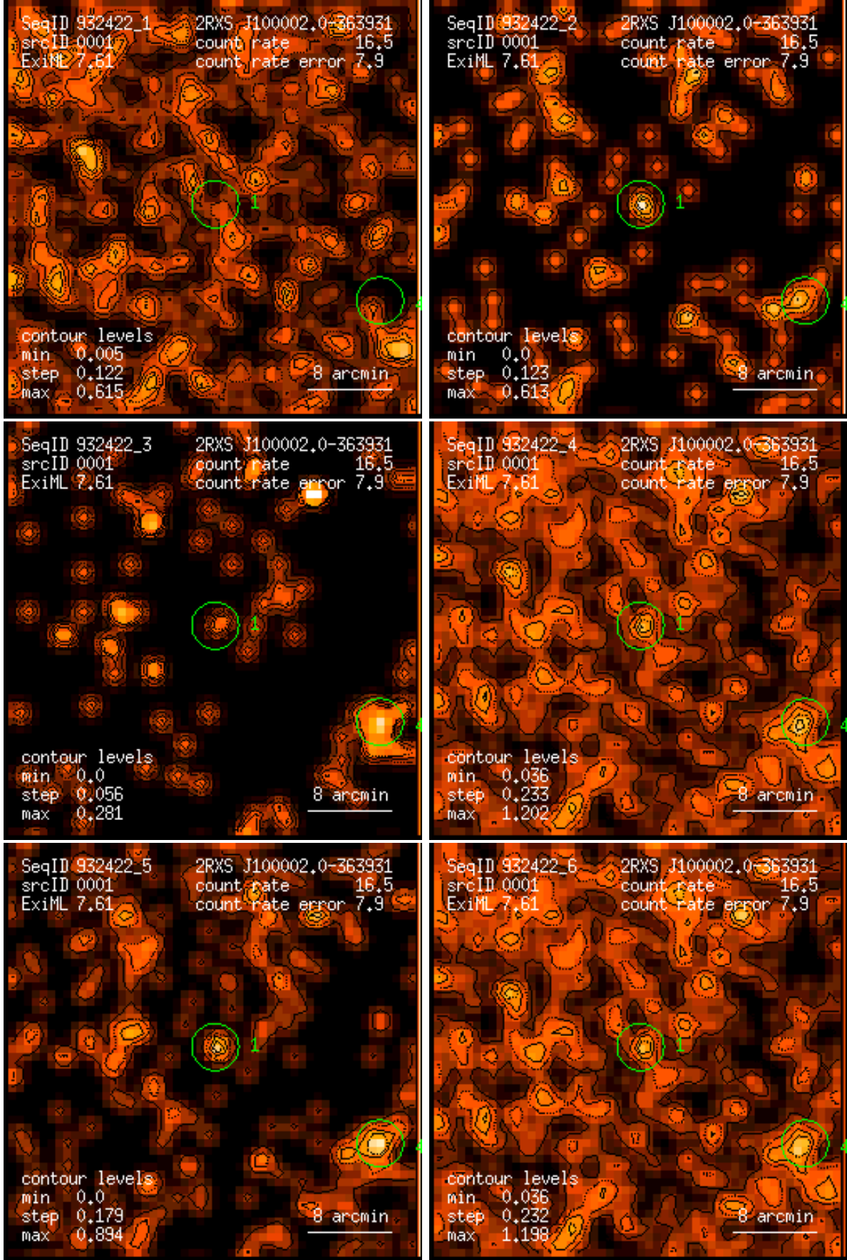
Figure 1: RASS 932422: detection 0001: band rate images, Gaussian filter: (1) PSPC channels 11 – 41, (2) 52 – 90, (3) 91 – 201, (4) 11 – 235, (5) 52 – 201, (6) 11 – 201. Broad band rates in counts/ks. Band rate contour levels in counts/ks/arcmin 2 .
