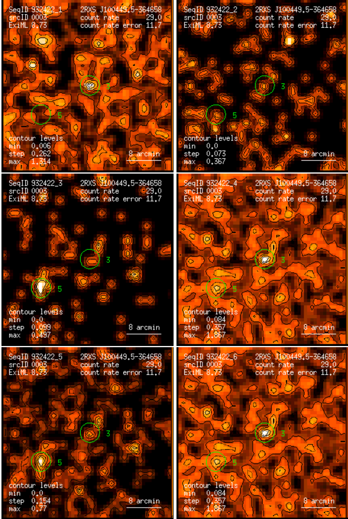
Figure 3: RASS 932422: detection 0003: band rate images, Gaussian filter: (1) PSPC channels 11 – 41, (2) 52 – 90, (3) 91 – 201, (4) 11 – 235, (5) 52 – 201, (6) 11 – 201. Broad band rates in counts/ks. Band rate contour levels in counts/ks/arcmin 2 .
