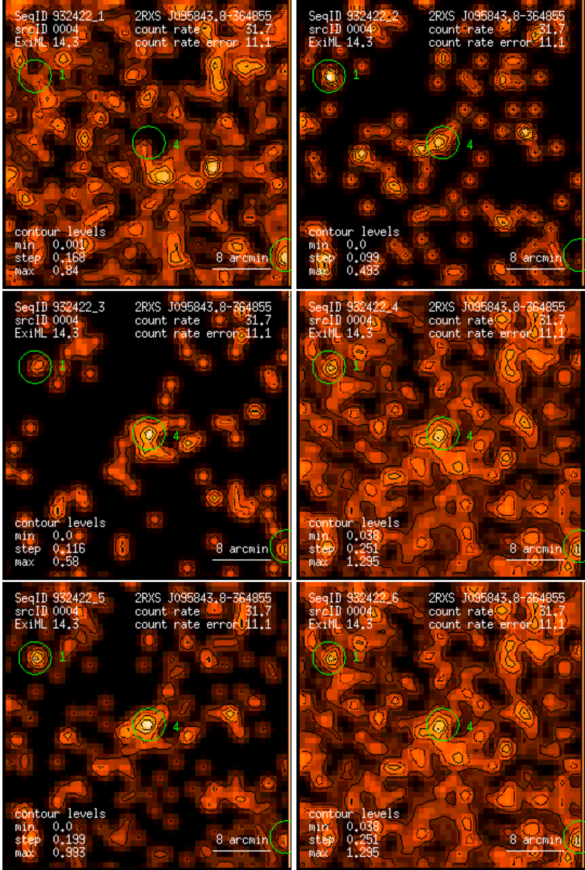
Figure 4: RASS 932422: detection 0004: band rate images, Gaussian filter: (1) PSPC channels 11 – 41, (2) 52 – 90, (3) 91 – 201, (4) 11 – 235, (5) 52 – 201, (6) 11 – 201. Broad band rates in counts/ks. Band rate contour levels in counts/ks/arcmin 2 .
