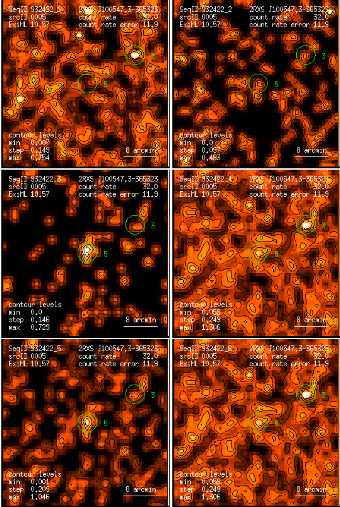
Figure 5: RASS 932422: detection 0005: band rate images, Gaussian filter: (1) PSPC channels 11 – 41, (2) 52 – 90, (3) 91 – 201, (4) 11 – 235, (5) 52 – 201, (6) 11 – 201. Broad band rates in counts/ks. Band rate contour levels in counts/ks/arcmin 2 .
