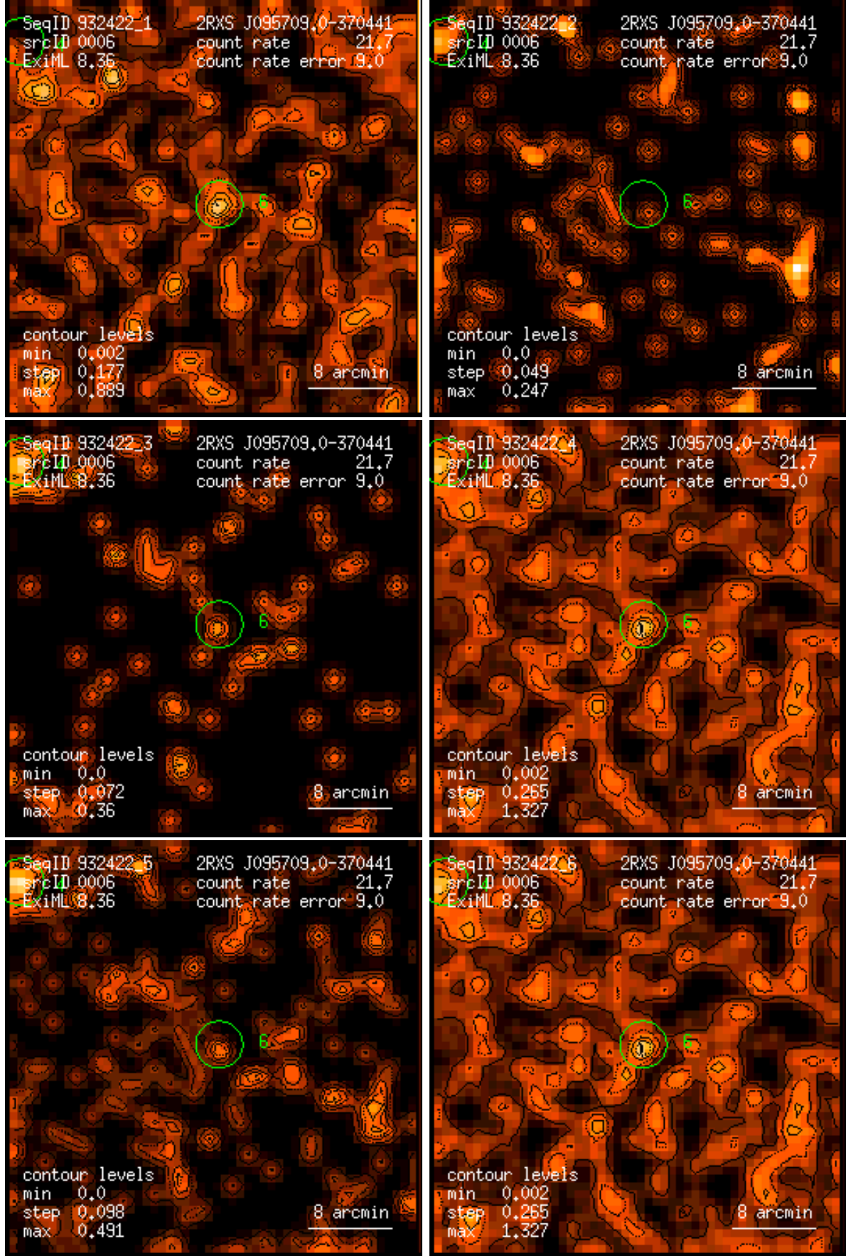
Figure 6: RASS 932422: detection 0006: band rate images, Gaussian filter: (1) PSPC channels 11 – 41, (2) 52 – 90, (3) 91 – 201, (4) 11 – 235, (5) 52 – 201, (6) 11 – 201. Broad band rates in counts/ks. Band rate contour levels in counts/ks/arcmin 2 .
