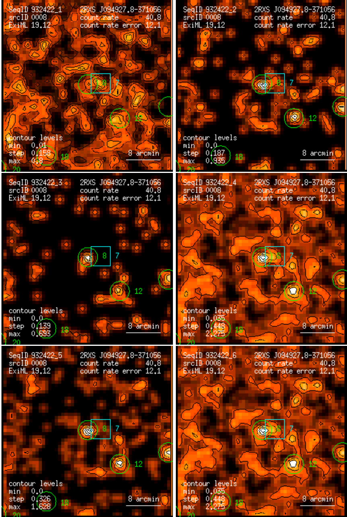
Figure 8: RASS 932422: detection 0008: band rate images, Gaussian filter: (1) PSPC channels 11 – 41, (2) 52 – 90, (3) 91 – 201, (4) 11 – 235, (5) 52 – 201, (6) 11 – 201. Broad band rates in counts/ks. Band rate contour levels in counts/ks/arcmin 2 .
