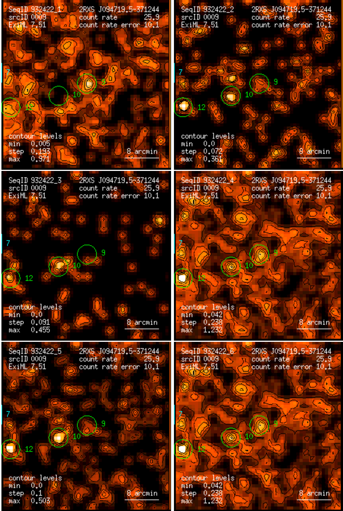
Figure 9: RASS 932422: detection 0009: band rate images, Gaussian filter: (1) PSPC channels 11 – 41, (2) 52 – 90, (3) 91 – 201, (4) 11 – 235, (5) 52 – 201, (6) 11 – 201. Broad band rates in counts/ks. Band rate contour levels in counts/ks/arcmin 2 .
