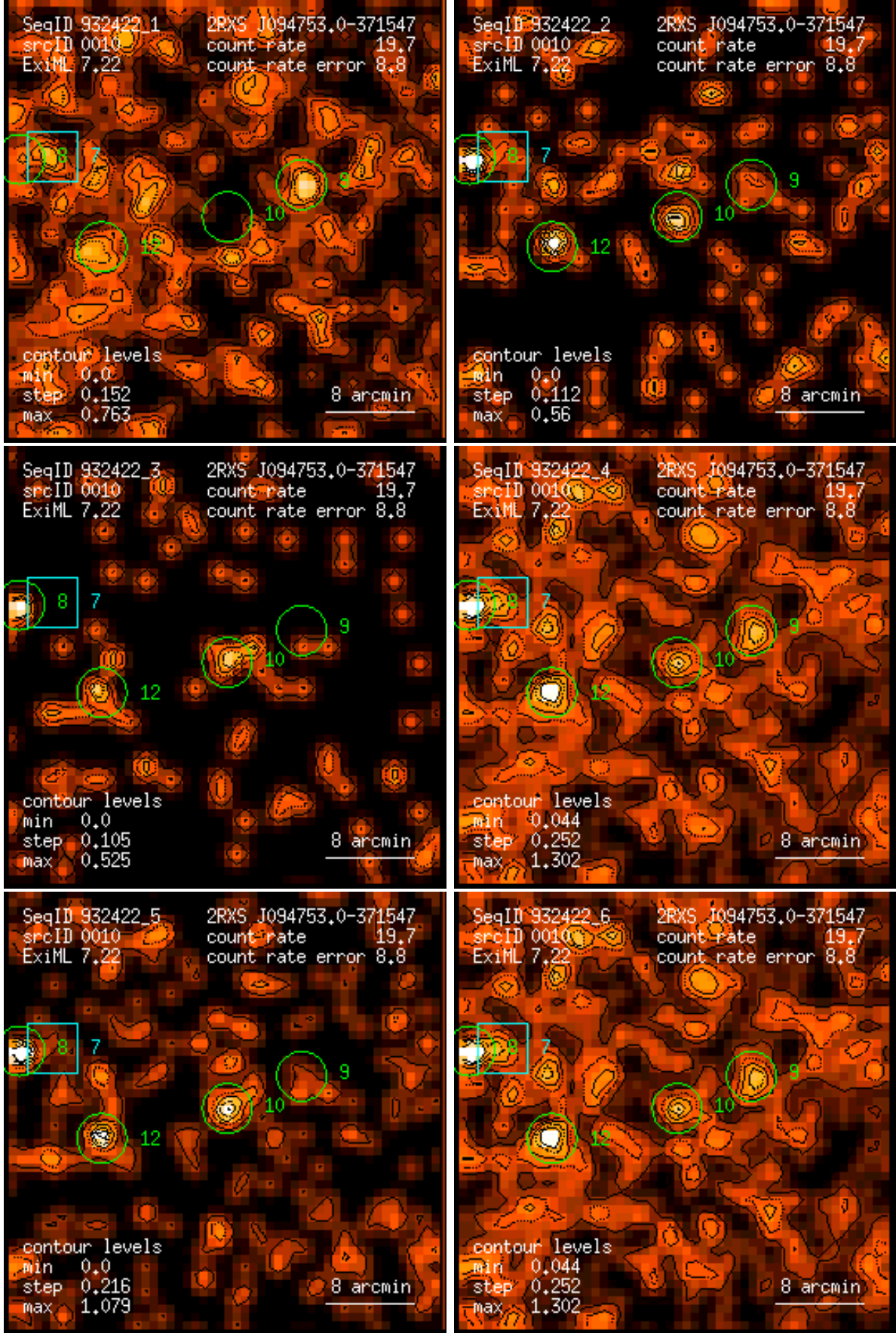
Figure 10: RASS 932422: detection 0010: band rate images, Gaussian filter: (1) PSPC channels 11 – 41, (2) 52 – 90, (3) 91 – 201, (4) 11 – 235, (5) 52 – 201, (6) 11 – 201. Broad band rates in counts/ks. Band rate contour levels in counts/ks/arcmin 2 .
